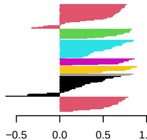
k = 13
