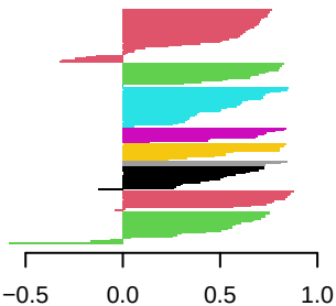
k = 14
