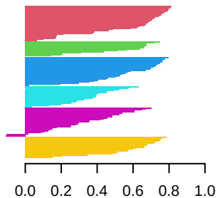
k = 10
