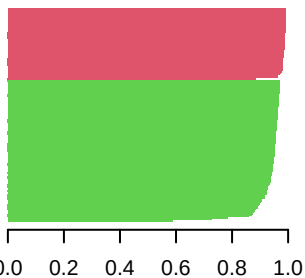
k = 6
