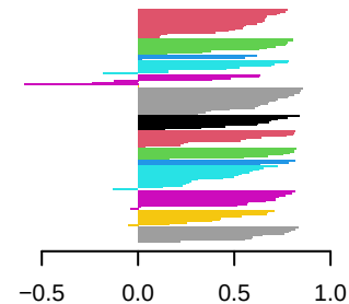
k = 15
