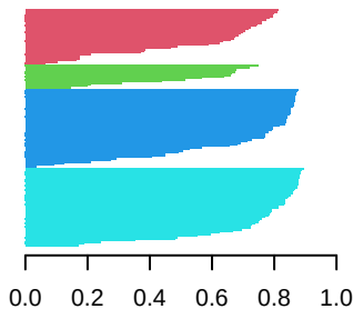
k = 8
