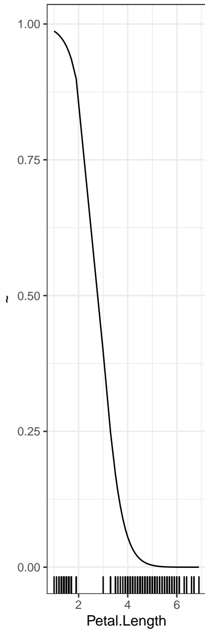
PDP – setosa
