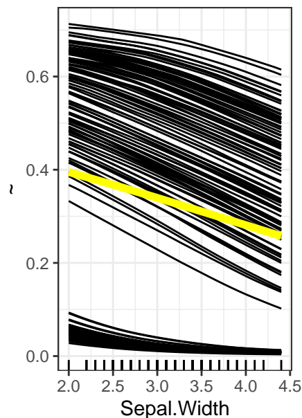
PDP – virginica
