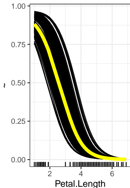
PDP – setosa
