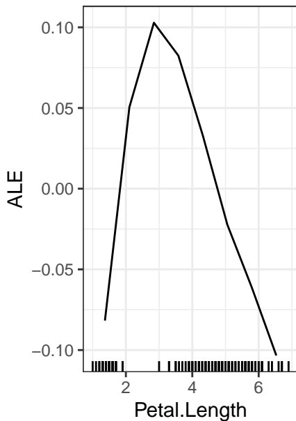
Petal.Length ... versic
