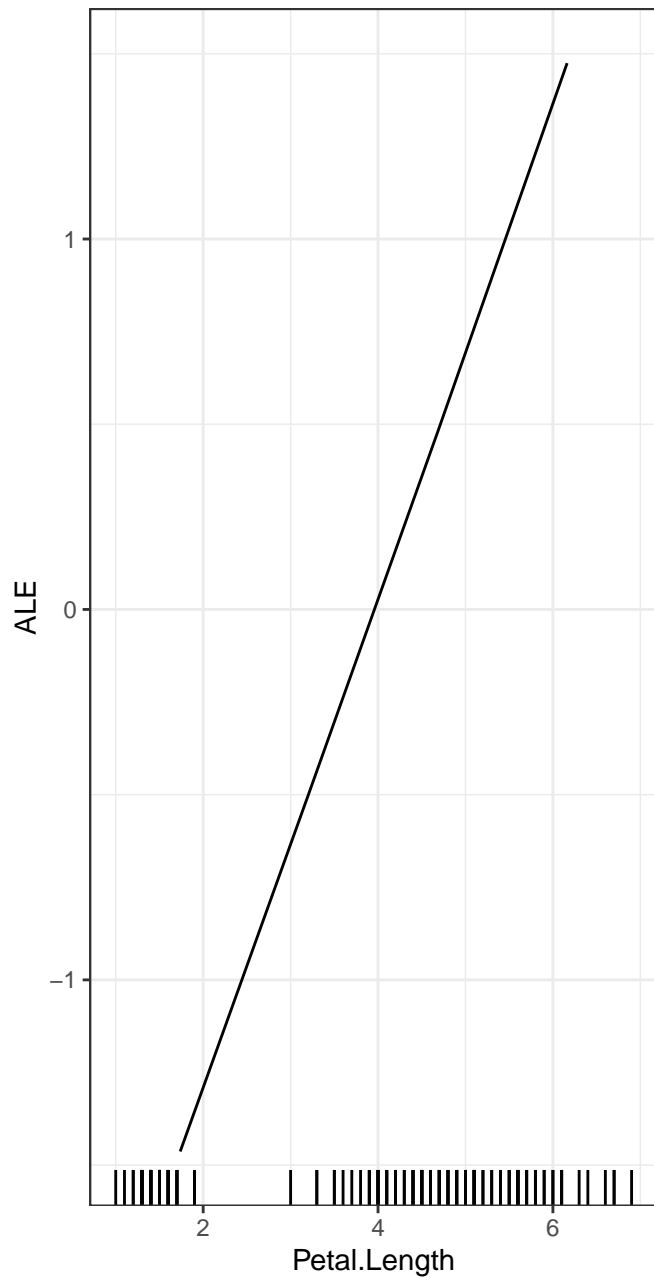
Petal.Length ... Sepal.Length
