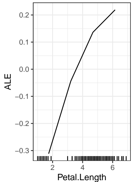
Petal.Length ... virginica
