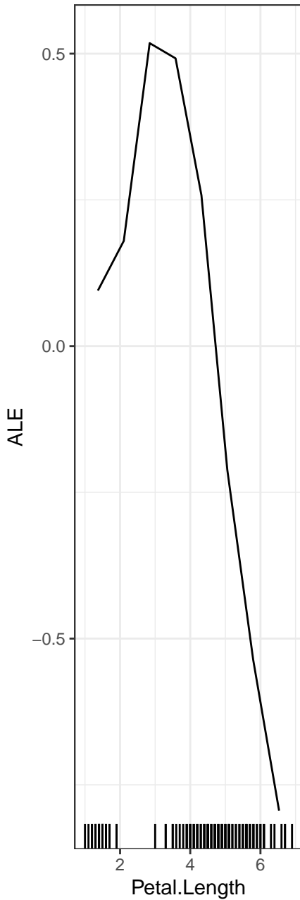
Petal.Length ... versicol
