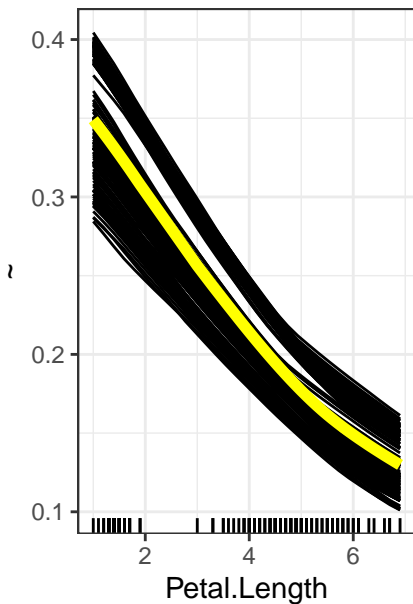
PDP – setosa
