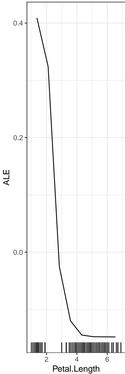
Petal.Length ... setosa
