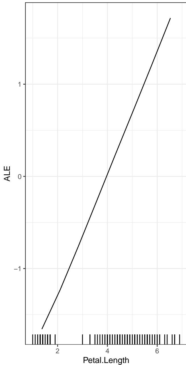
Petal.Length ... Sepal.Length
