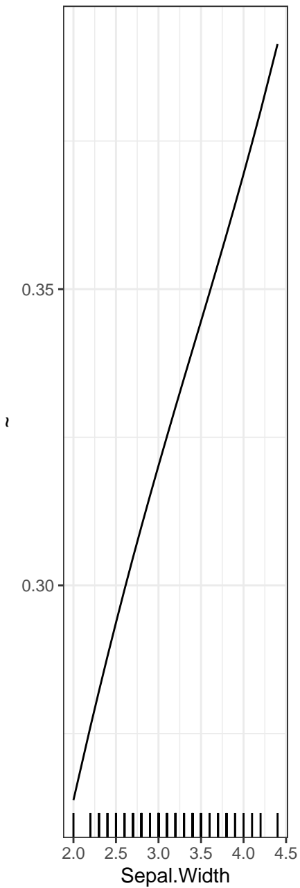
PDP – setosa
