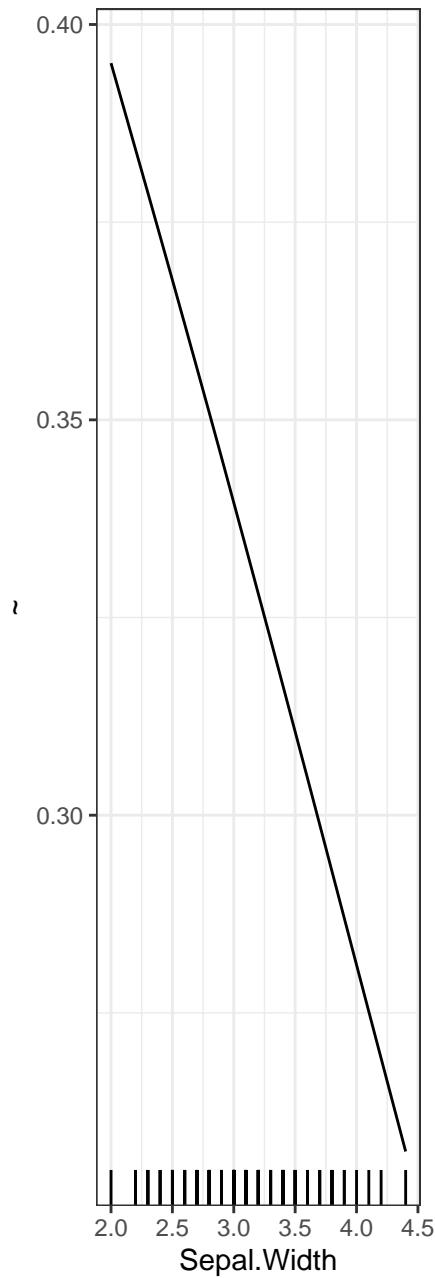
PDP – virginica
