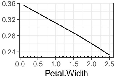
PDP – setosa
