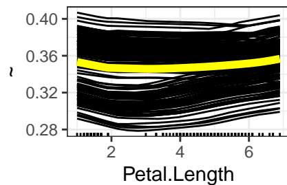
PDP – virginica
