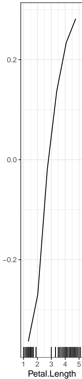
Petal.Length ...
