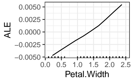
Petal.Width ... virgin
