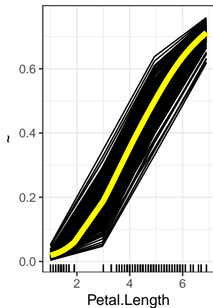
PDP – virginica
