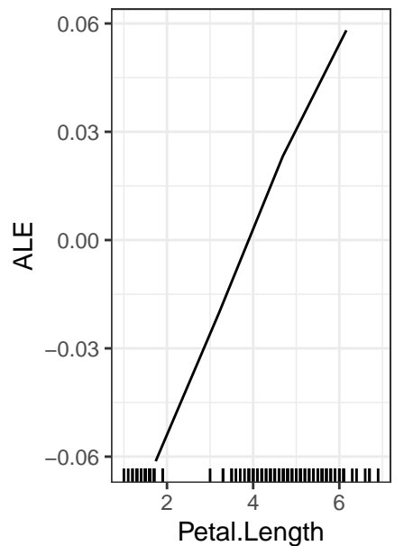
Petal.Length ... virgin
