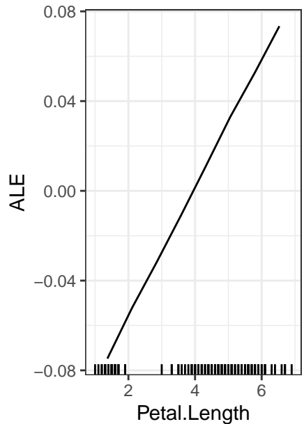
Petal.Length ... virgin
