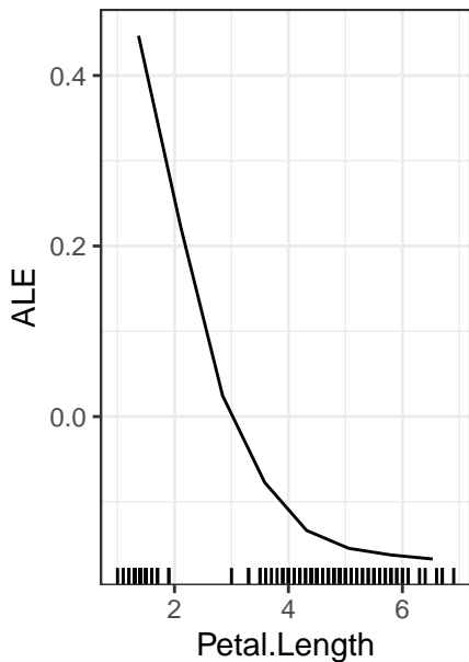
Petal.Length ... setosa
