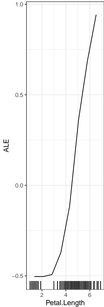
Petal.Length ... virginica
