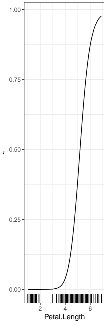
PDP – virginica
