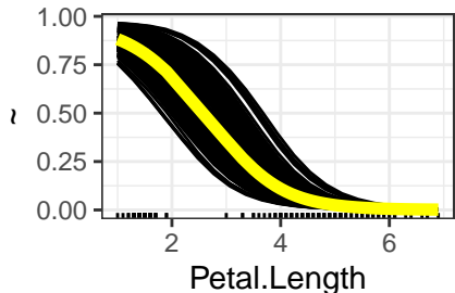
PDP – setosa
