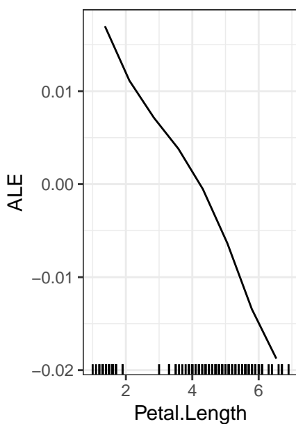
Petal.Length ... versic
