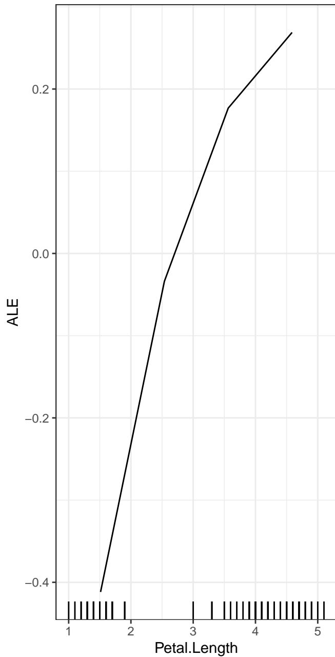
Petal.Length ... Species
