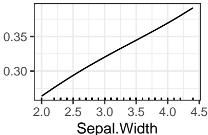
PDP – setosa
