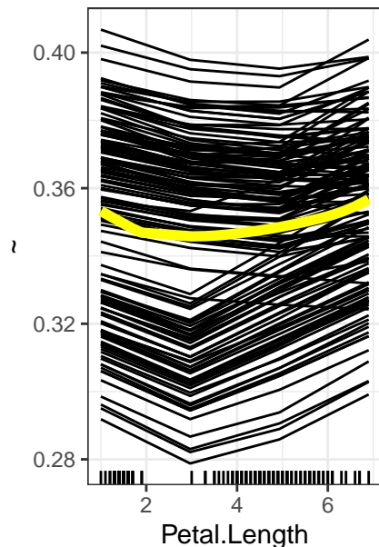
PDP – virginica
