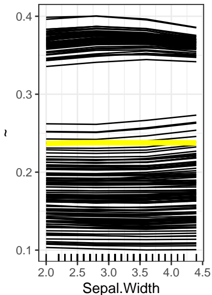
PDP – setosa
