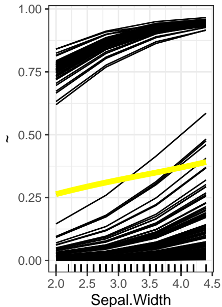
PDP – setosa
