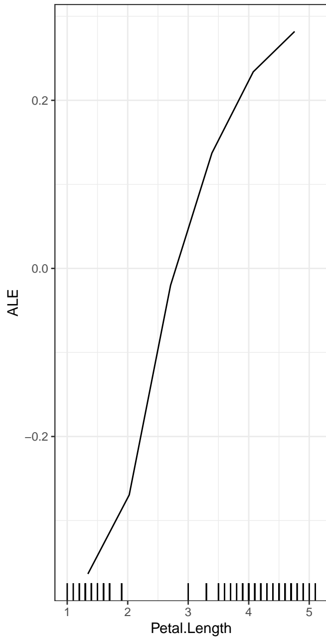
Petal.Length ... Species
