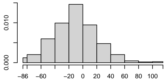
Density of istar2
