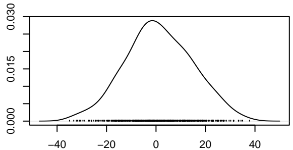
Density of edg cov.covariates
