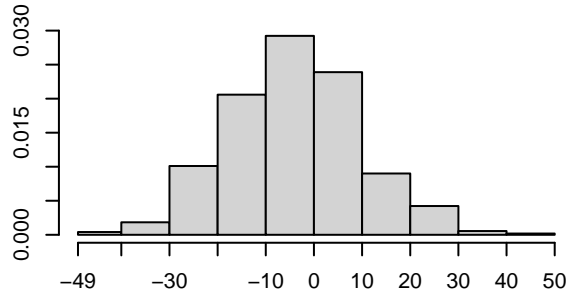
Density of edges
