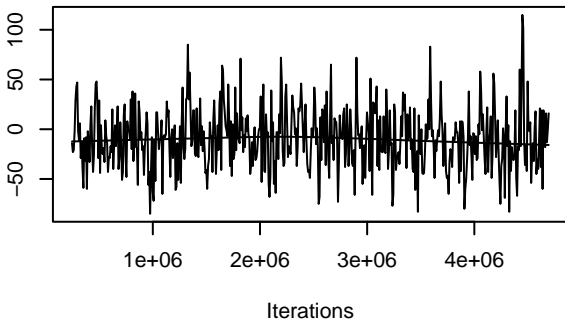
Trace of istar2
