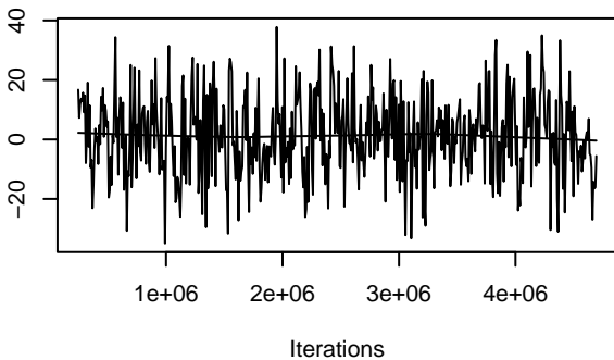
Trace of edg cov.covariates
