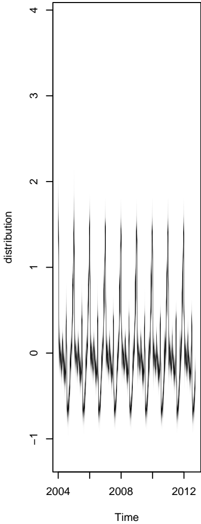
seasonal.52.1
