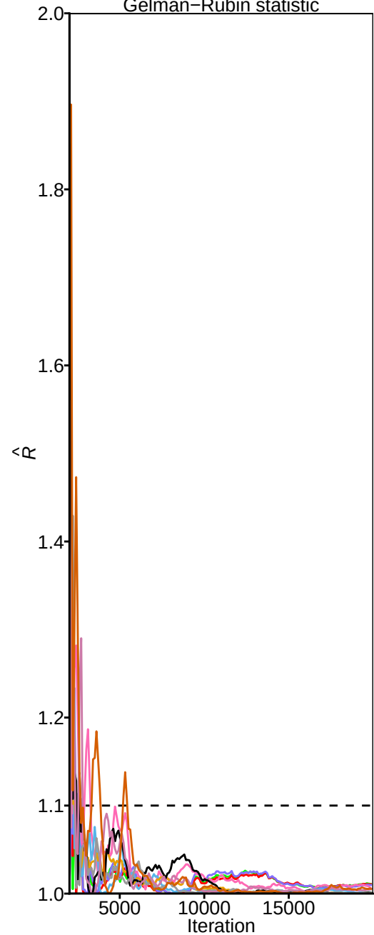
Gelman–Rubin statistic
