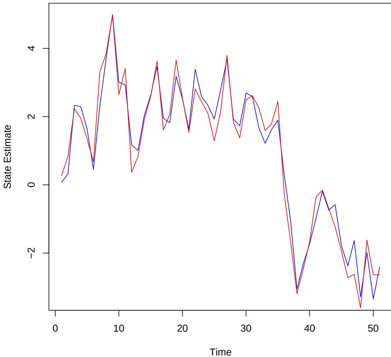
Particle Filter State Estimate vs True State
