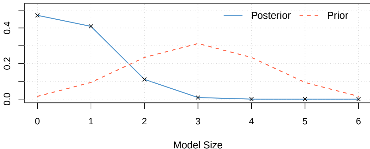
Posterior Model Size Distribution Mean: 0.658
