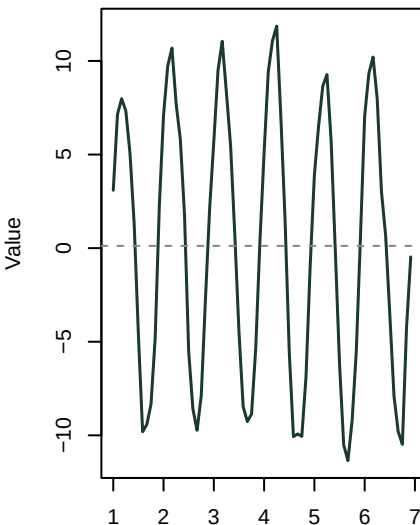
Time Plot
