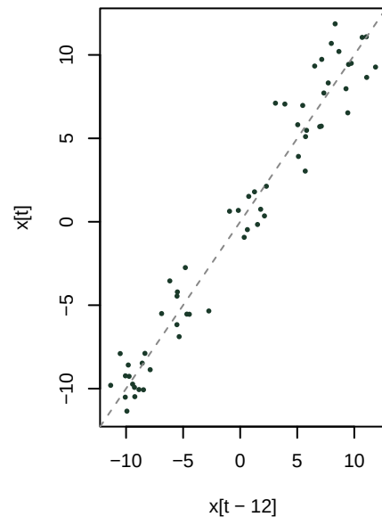
Seasonal Lag Plot
