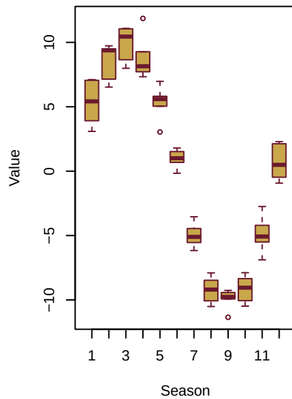
Seasonal Subseries
