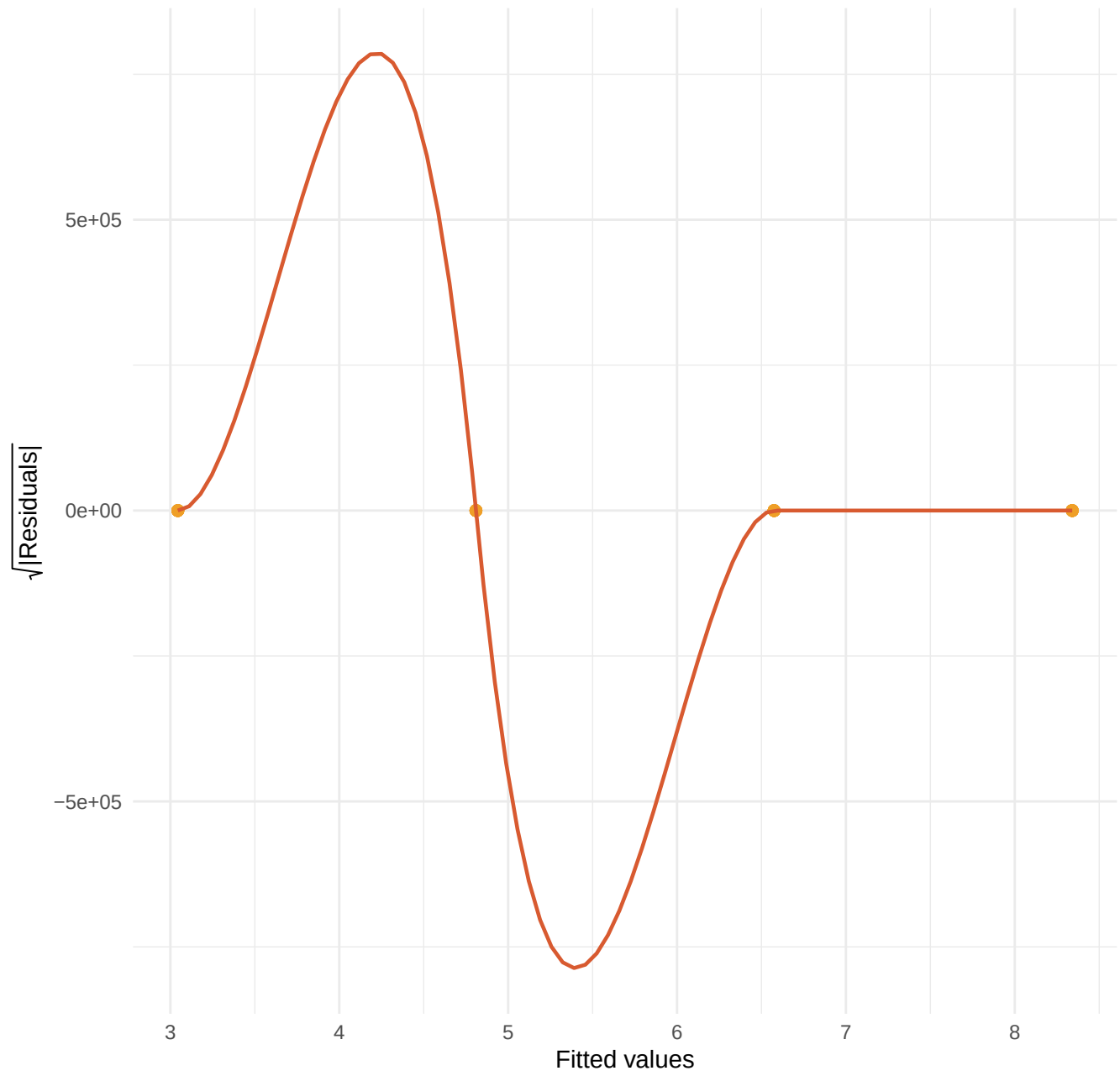
Scale-Location
