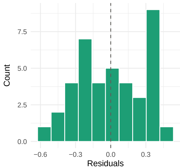
Residual histogram
