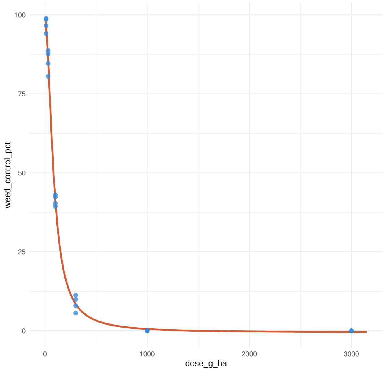
Dose-response curve: LL.4
