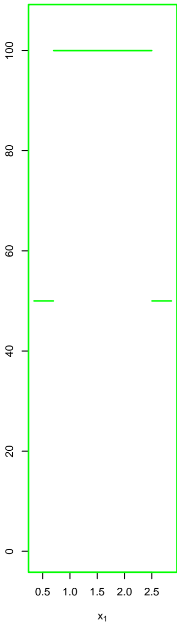
Group-wise sample size
