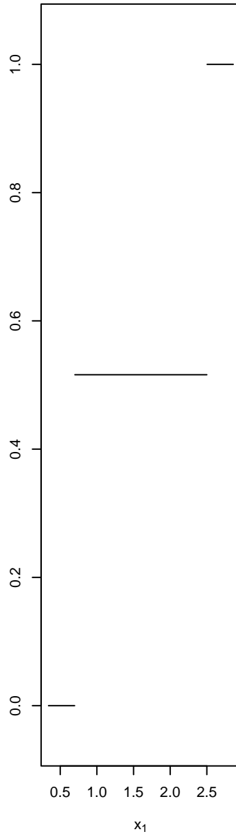
ConditionalPower
