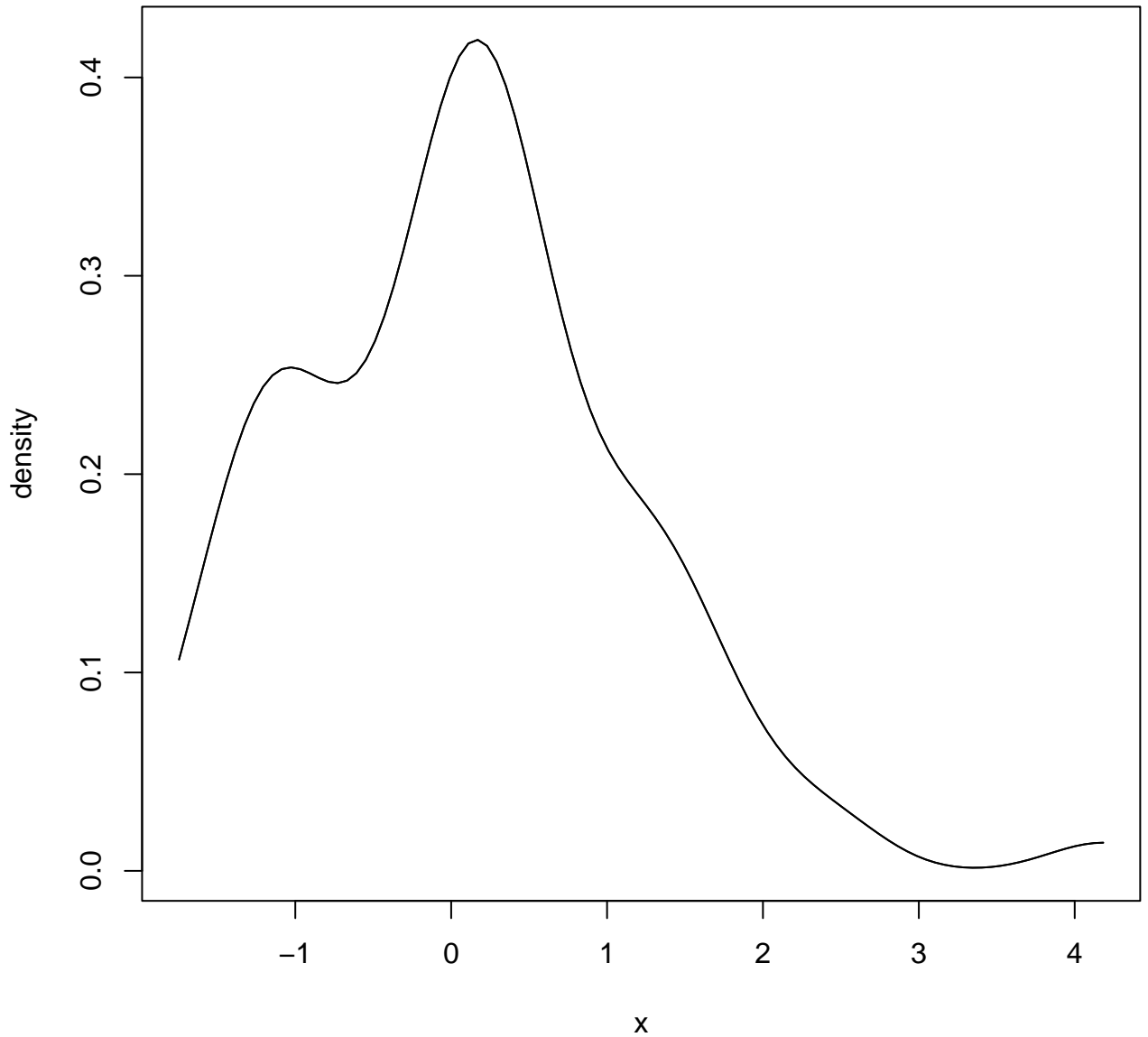
pdf of the unknown component
