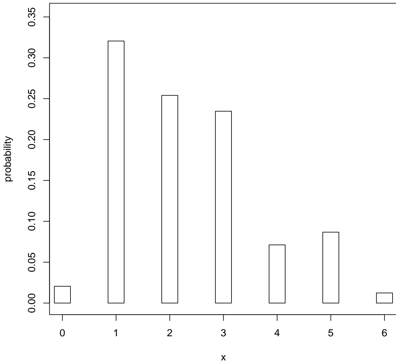
pmf of the unknown component
