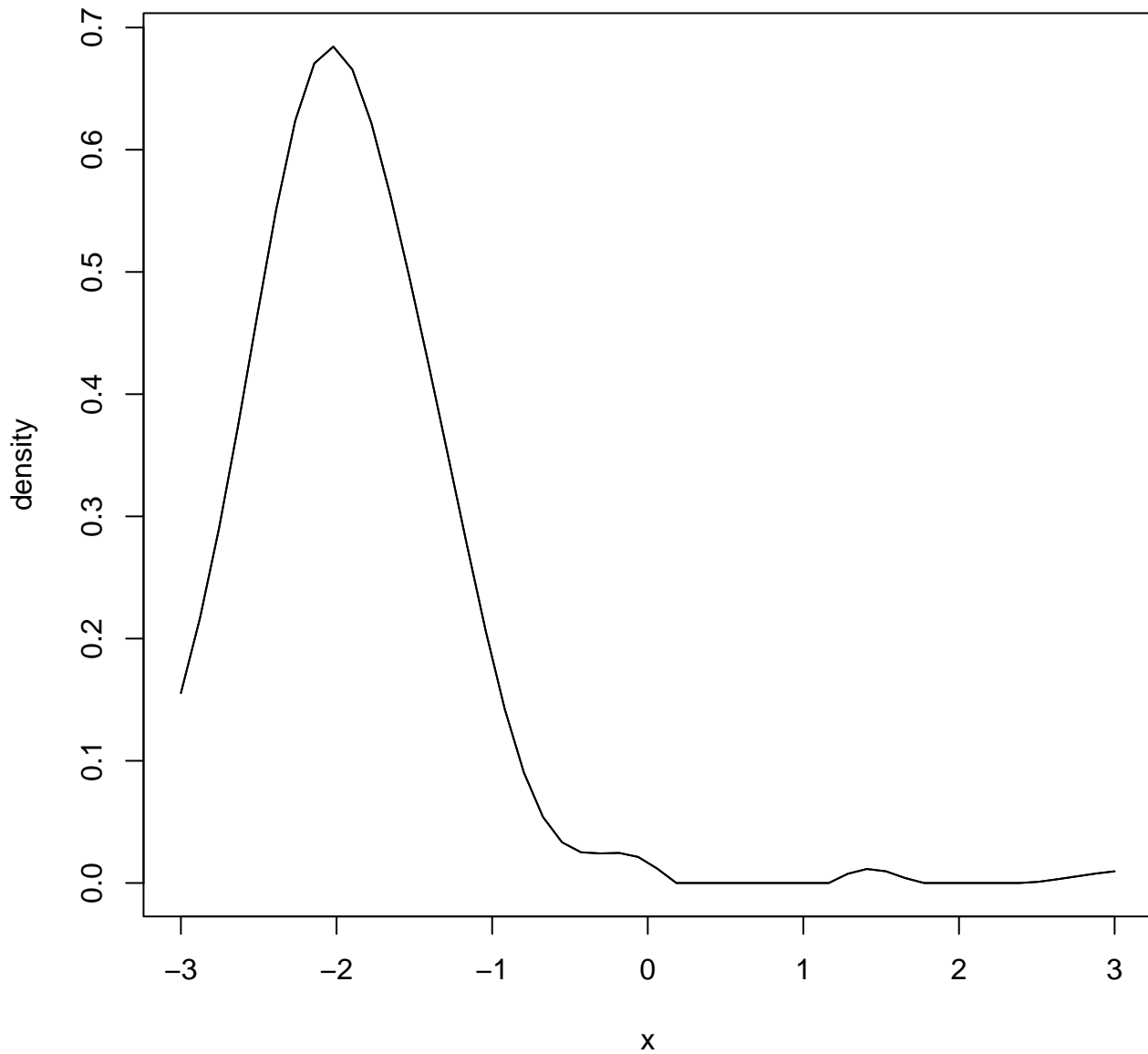
pdf of the unknown component
