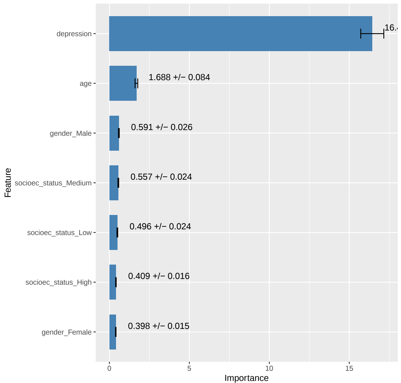
Mean |SHAP| value
