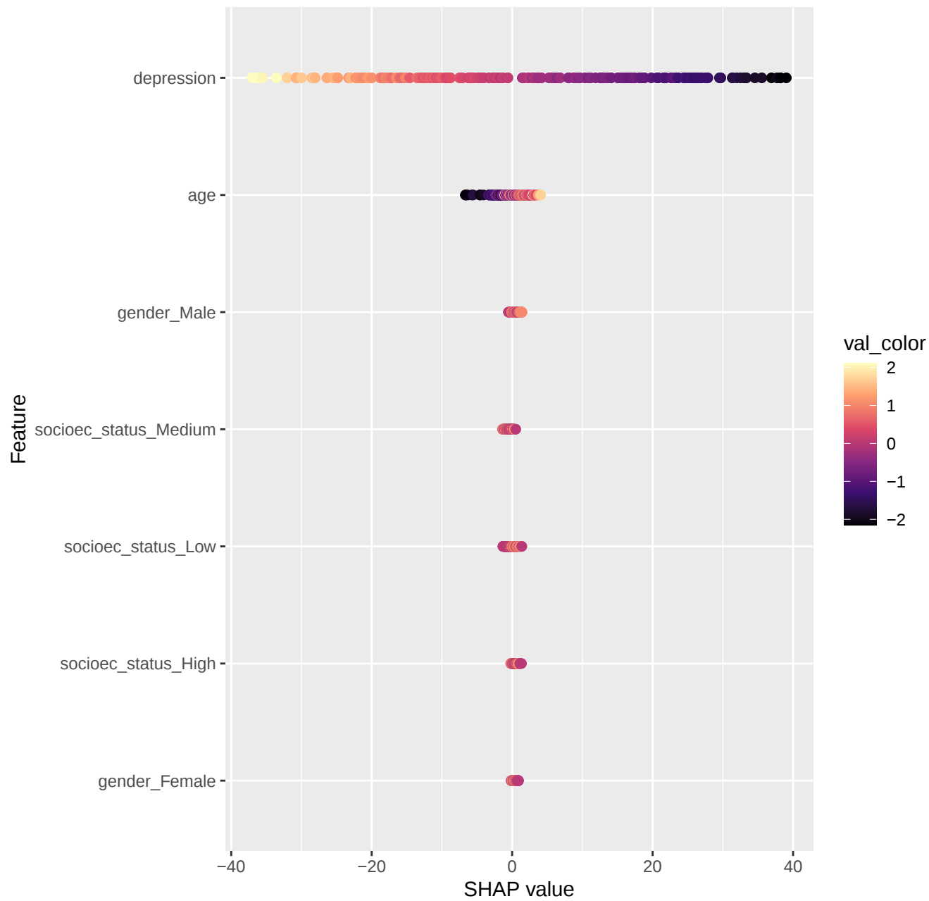
SHAP Swarm Plot
