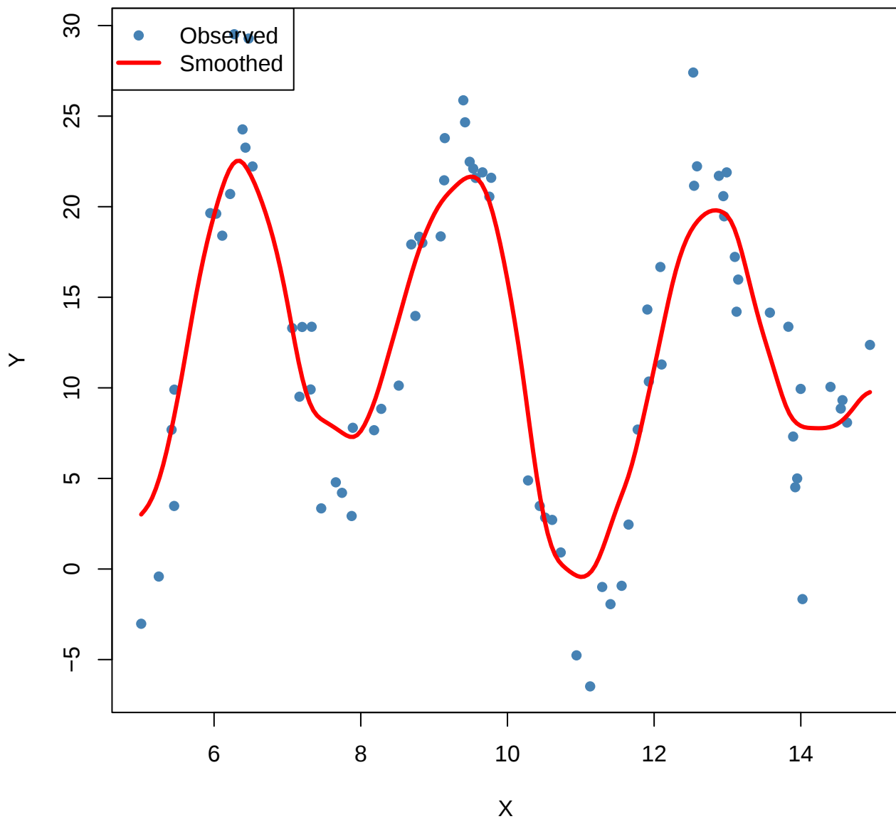
Kernel Regression Fit (tricube, h = 1 )
