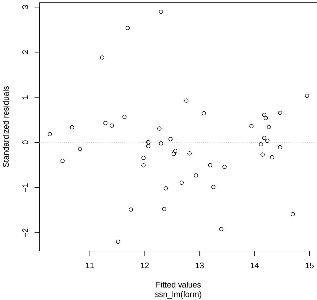
Standardized Residuals vs Fitted
