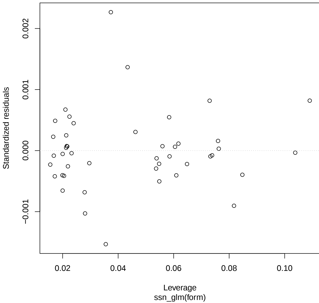
Standardized residuals vs Leverage
