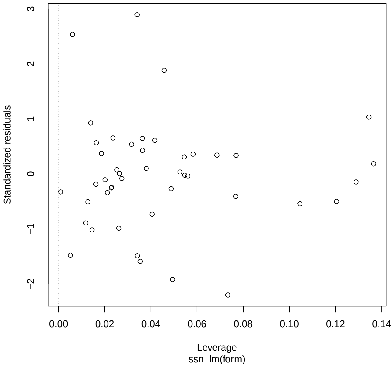
Standardized residuals vs Leverage
