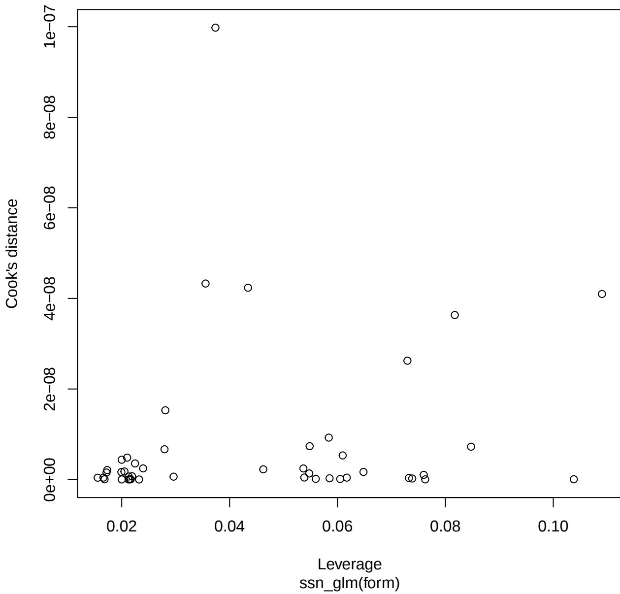
Cook's dist vs Leverage
