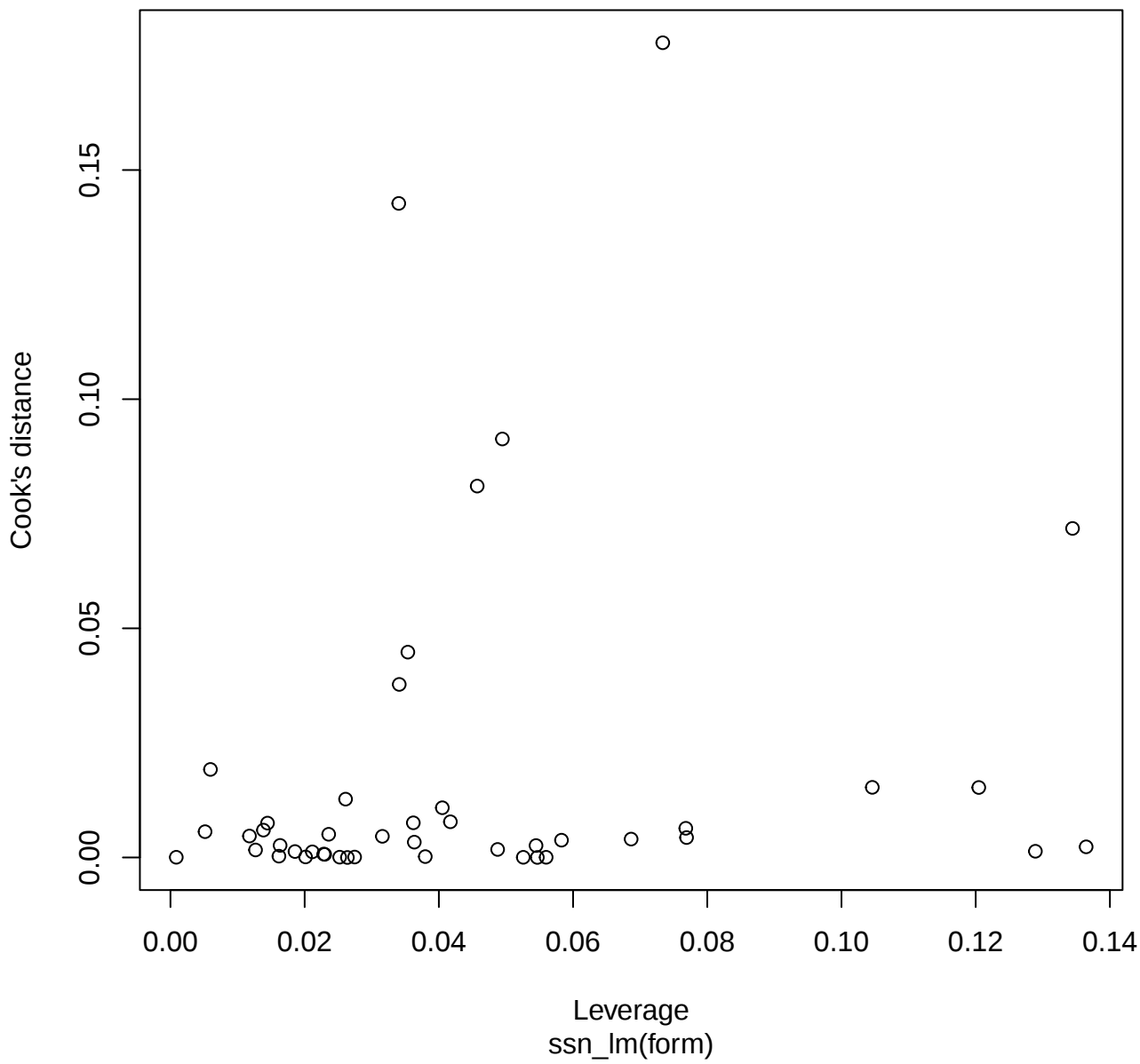
Cook's dist vs Leverage
