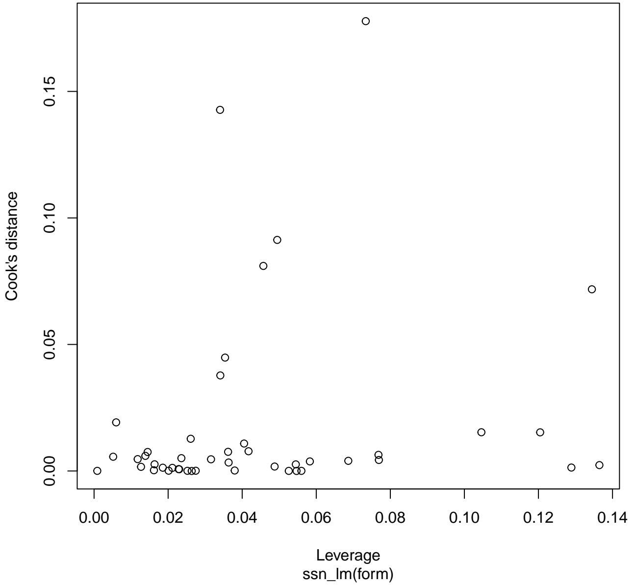
Cook's dist vs Leverage
