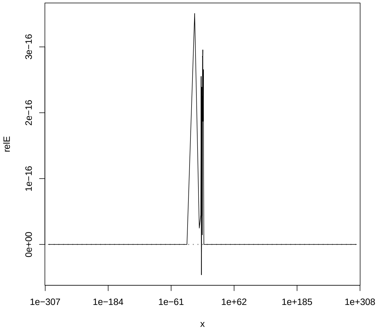
rel.Errors dgamma(., shape = 2^4)
