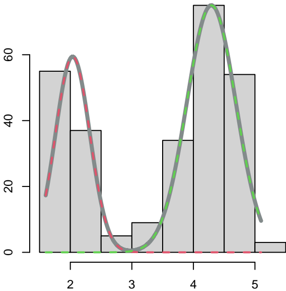
Histogram of Duration
