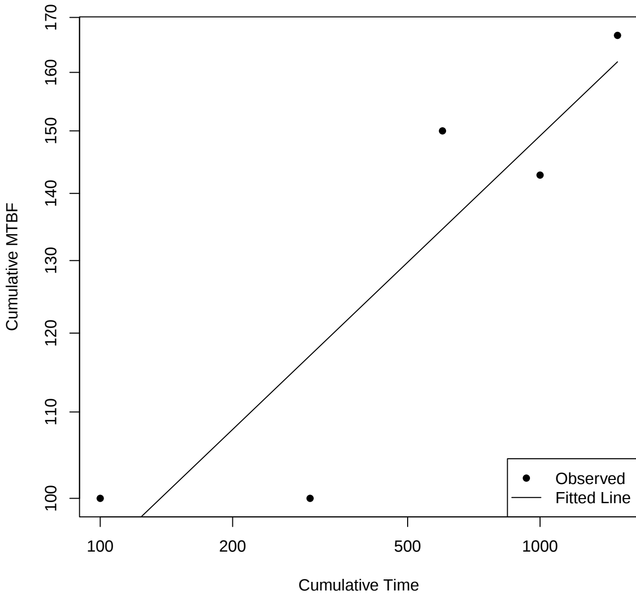
Duane Plot with Cumulative MTBF
