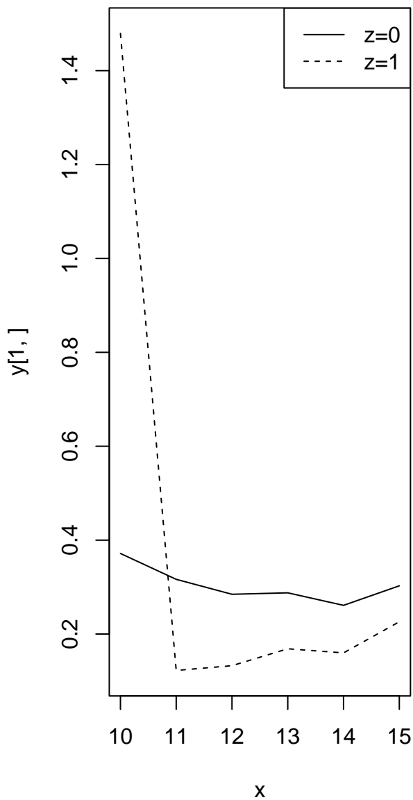
mean of eta estimate as a function of
