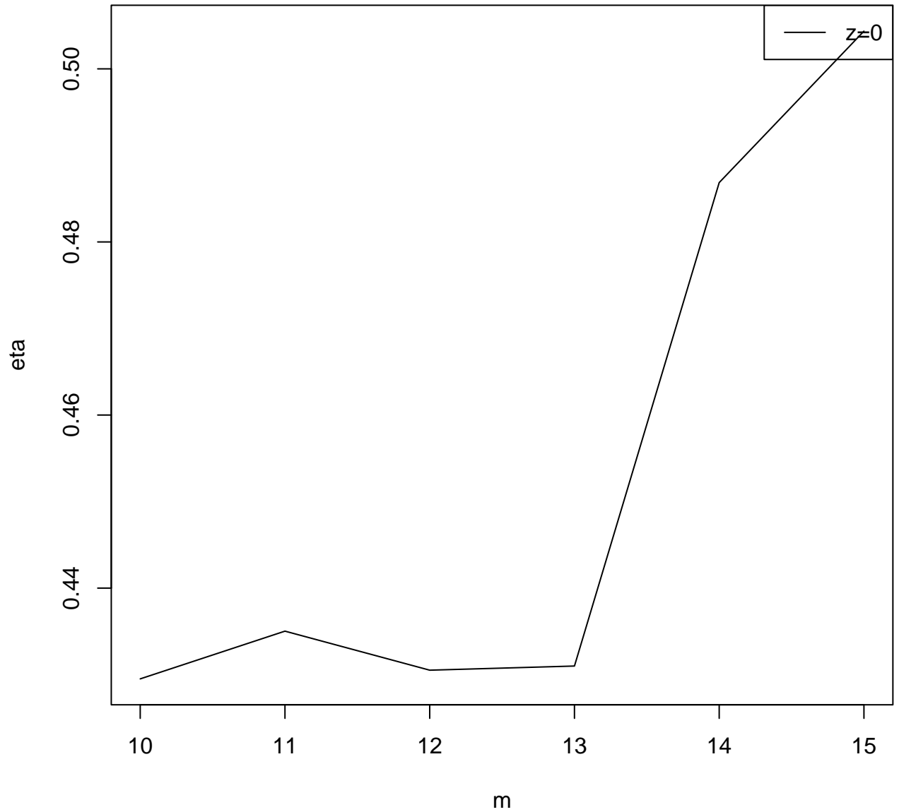
mean of eta estimate as a function of m
