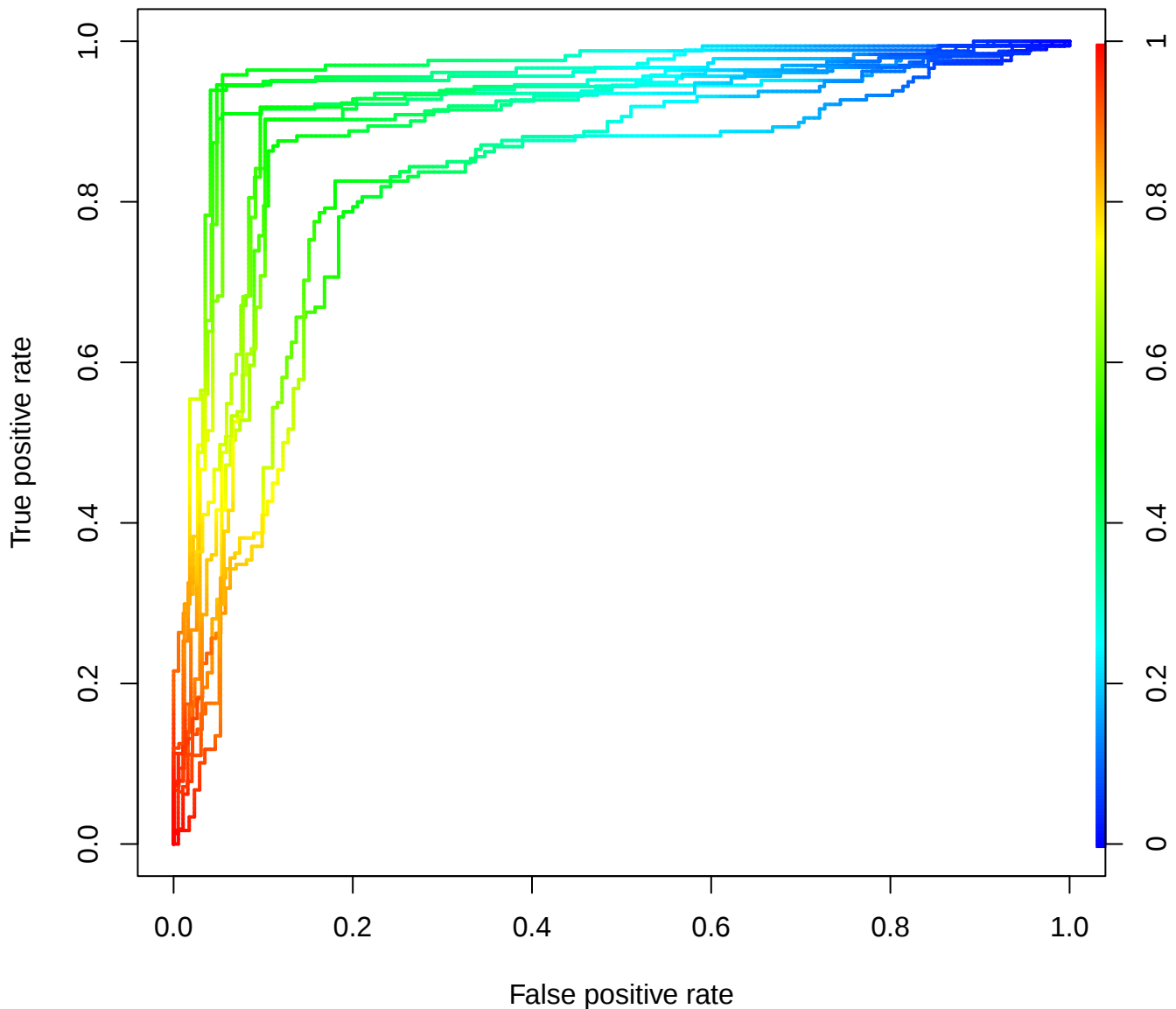
ROC curves from 10-fold cross-validation
