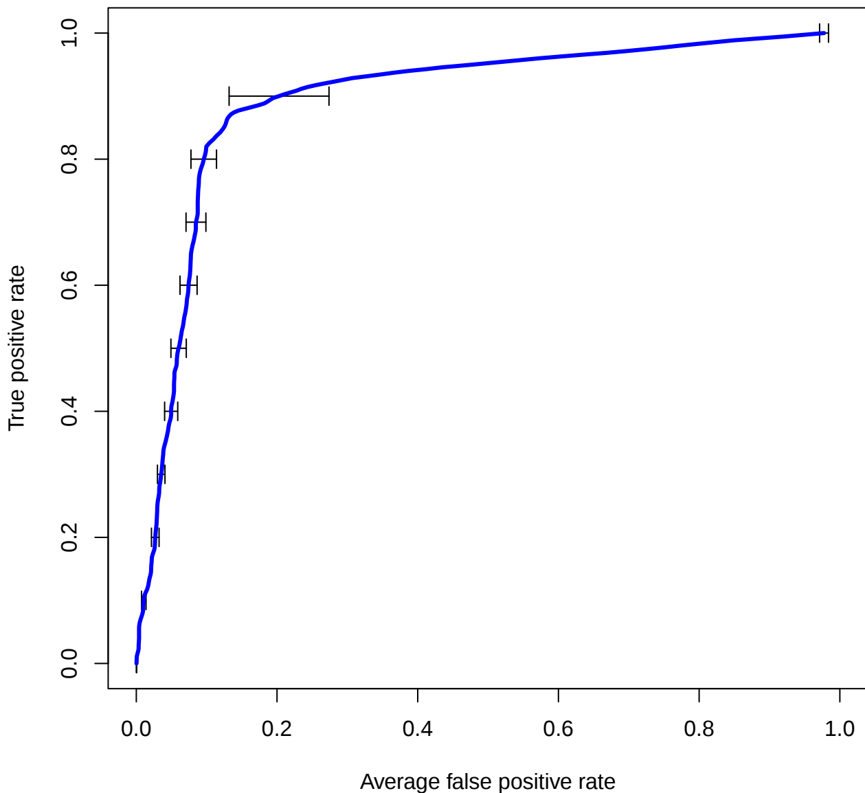
Horizontal averaging + boxplots
