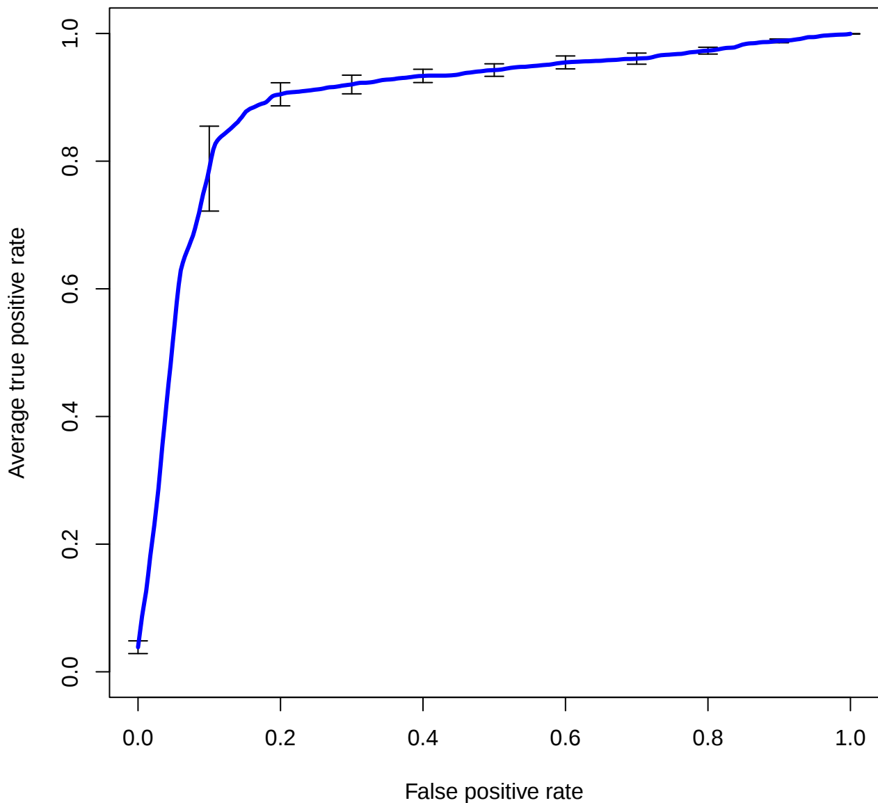
Vertical averaging + 1 standard error
