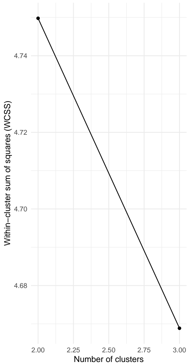
Euclidean
