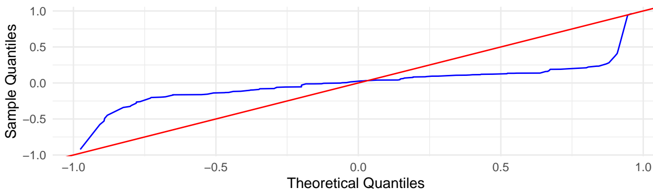
QQ Plot against Uniform – V3
