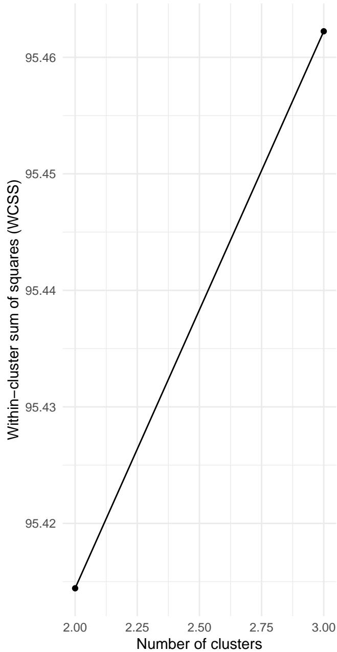
Cosine Similarity
