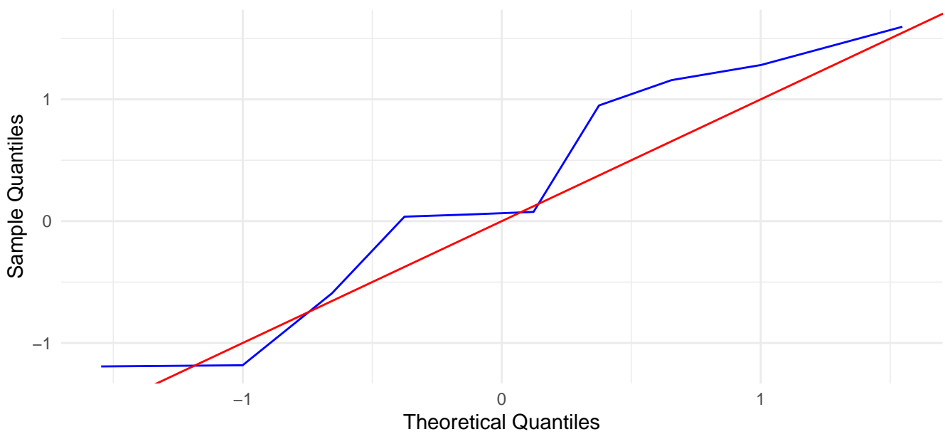
QQ Plot against Normal – V2
