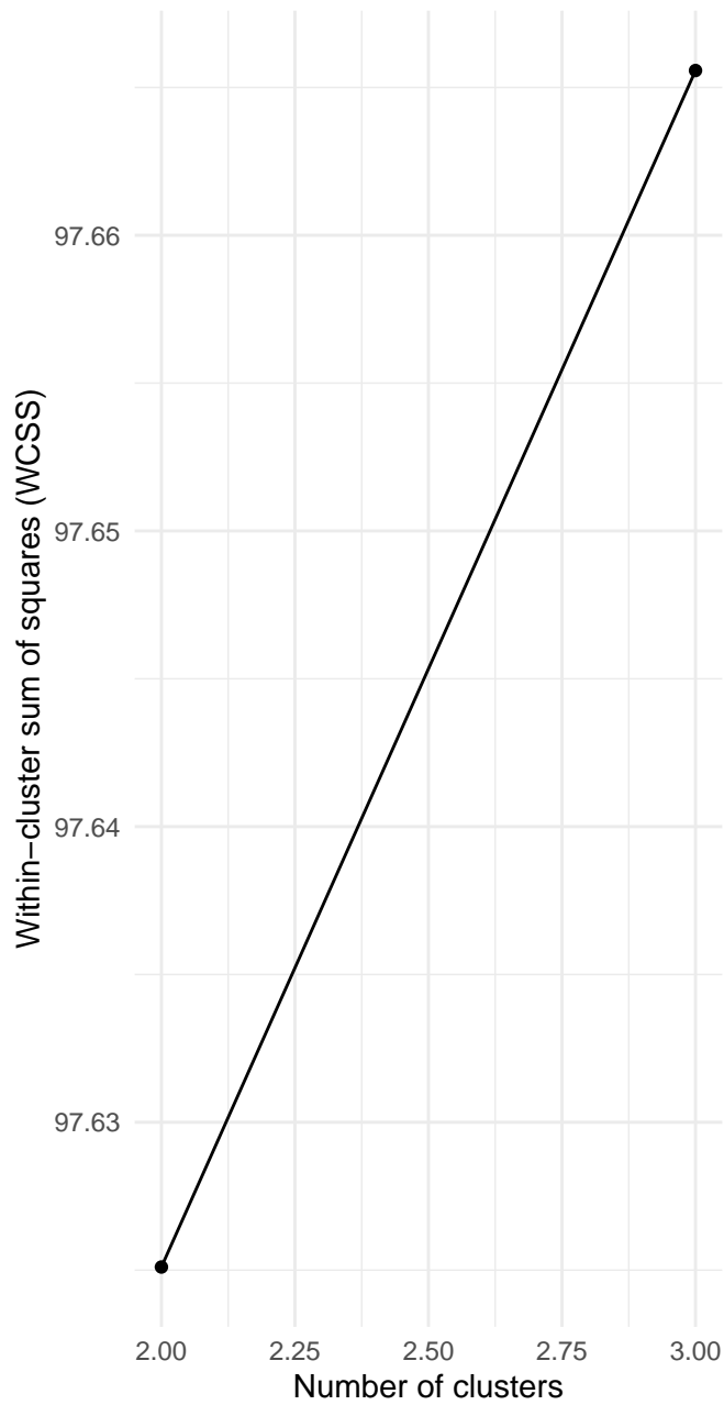
Cosine Similarity
