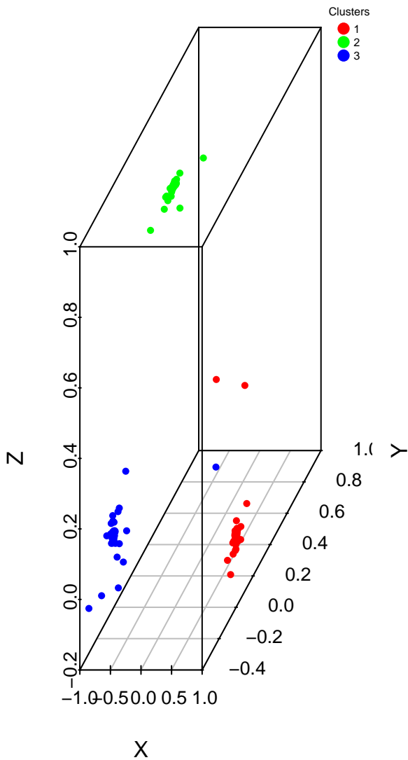
Final Membership
