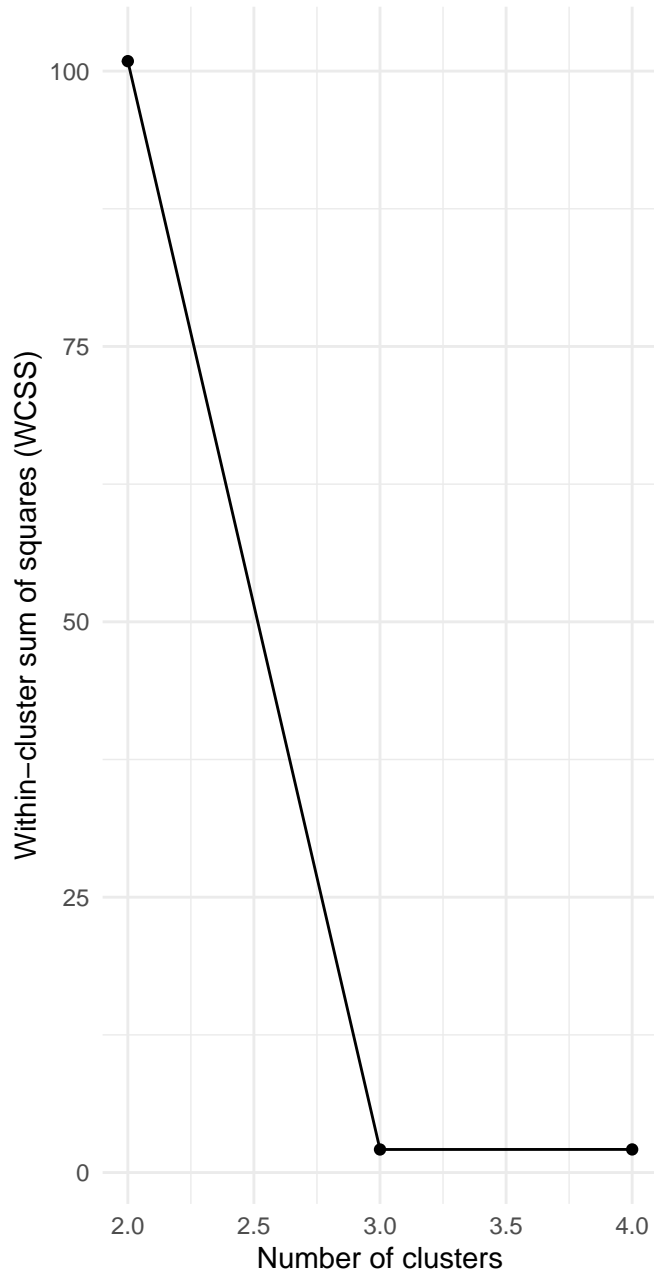
Euclidean
