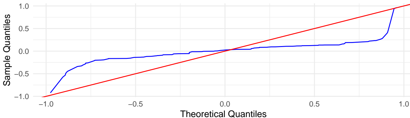
QQ Plot against Uniform – V2
