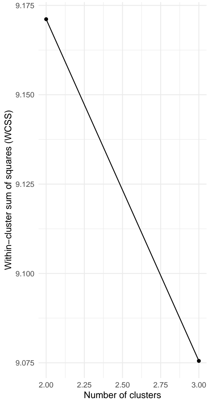
Euclidean
