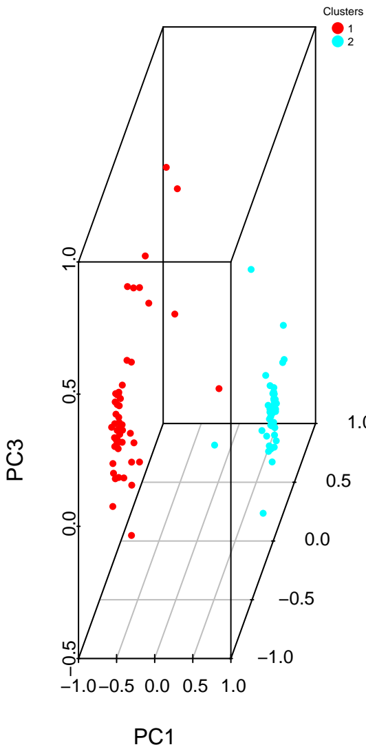
Final Membership
