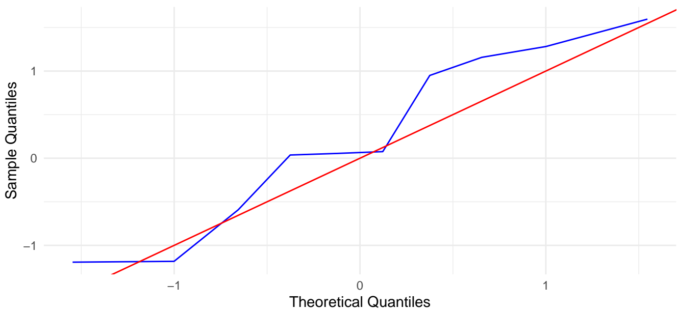
QQ Plot against Normal – V2
