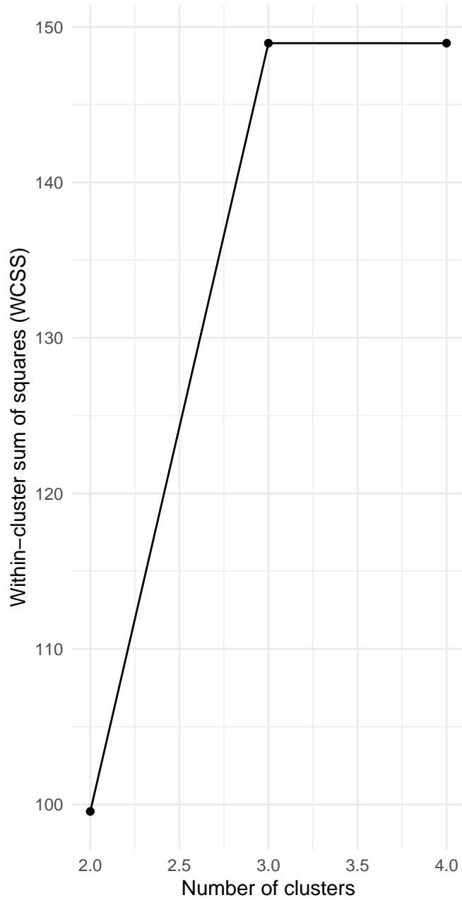
Cosine Similarity
