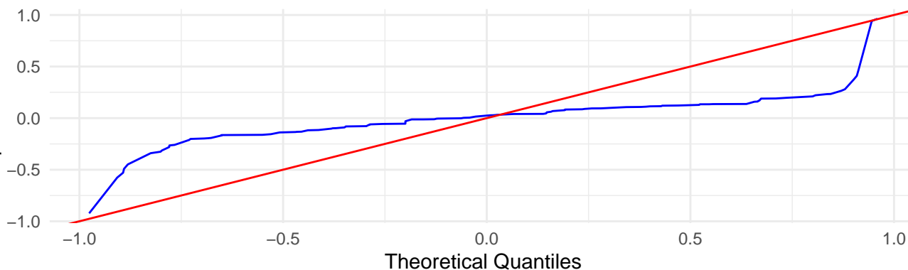
QQ Plot against Uniform – V3
