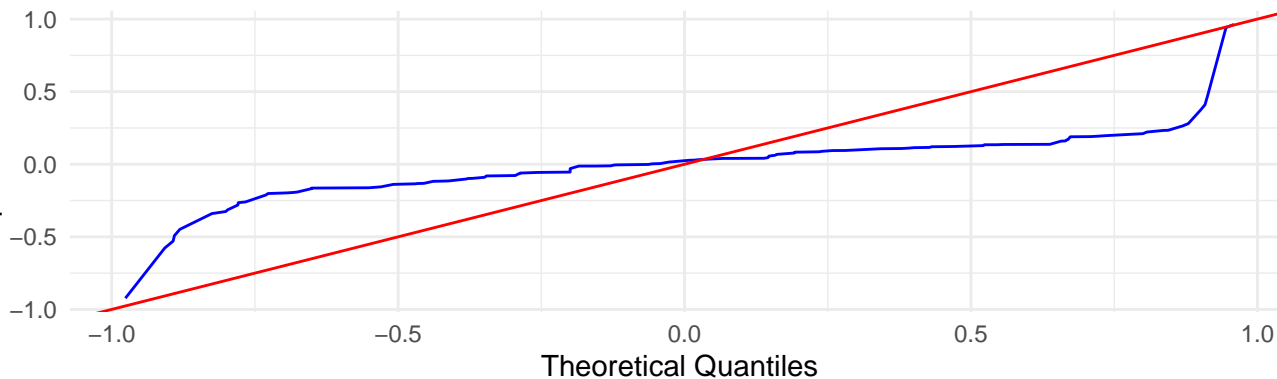
QQ Plot against Uniform – V2
