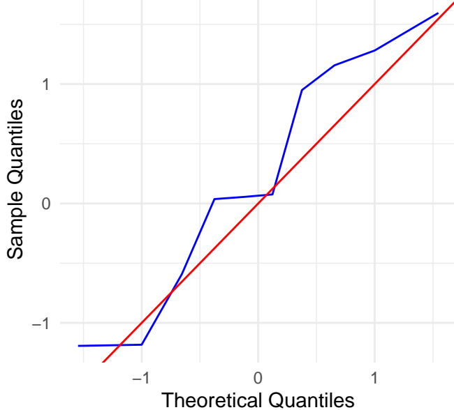
QQ Plot against Normal – V2
