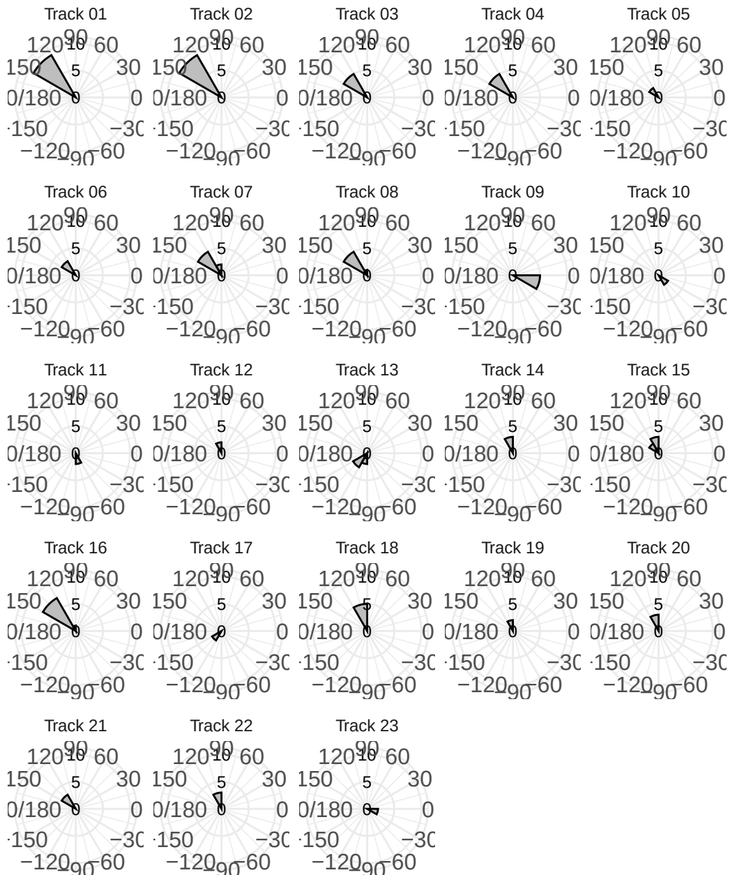
Direction (degrees) vs Trackways count
