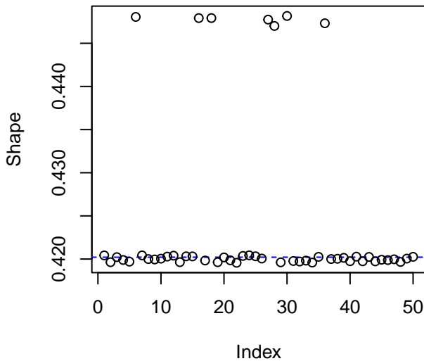
Shape Trace Plot
