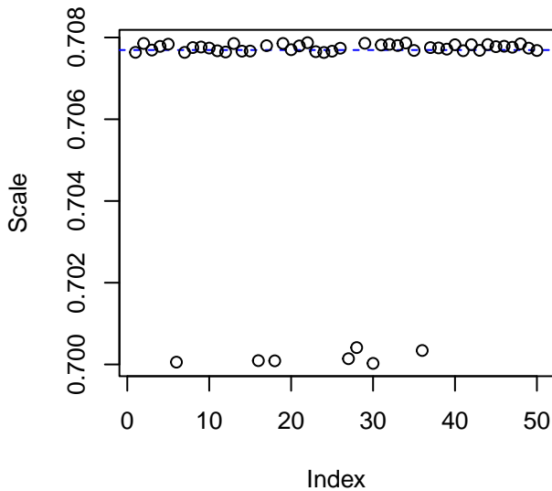
Scale Trace Plot
