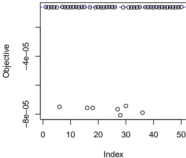
Objective Value Trace Plot
