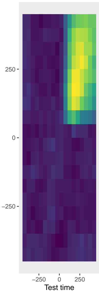
Zero-one loss
