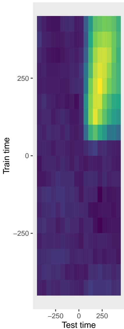
Zero-one loss
