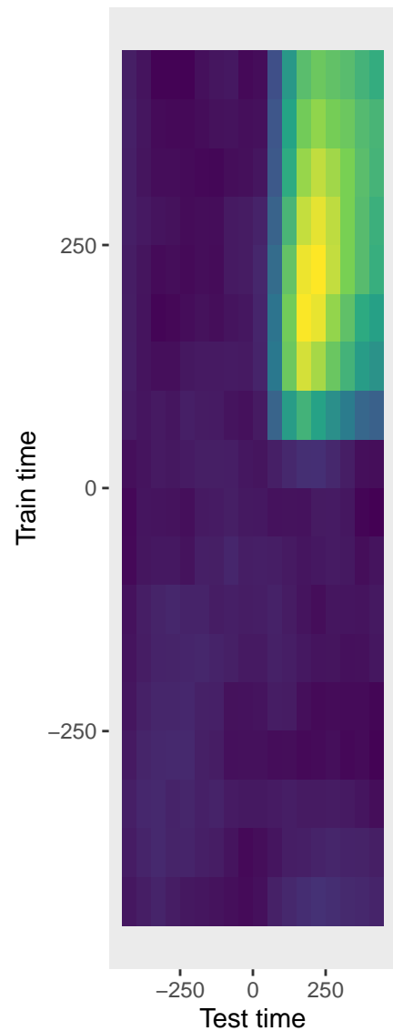
Decision values
