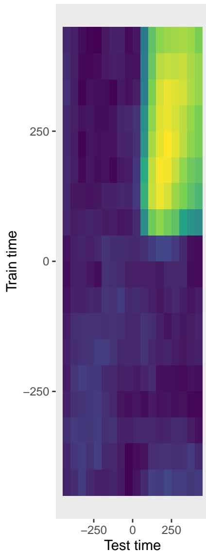
Normalized rank
