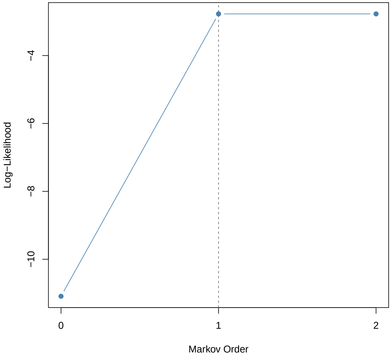
MOGen: Log-Likelihood by Order
