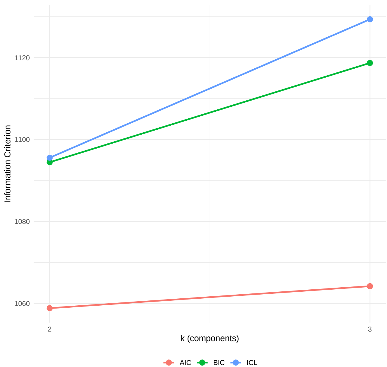
MMM Model Selection
