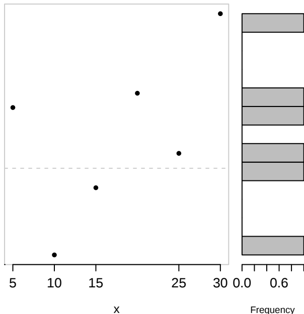
Residual plot
