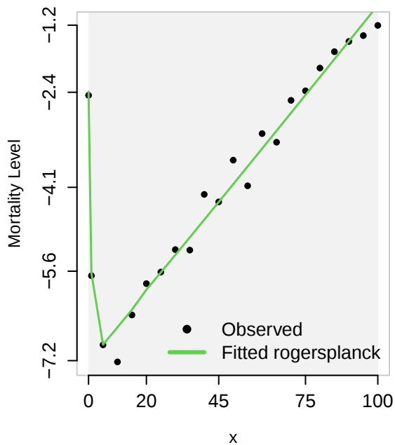
Observed vs. Fitted Rogers-Planck law
