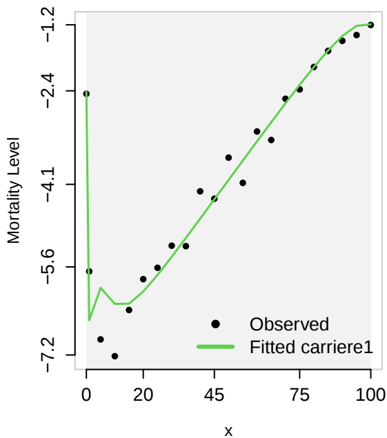
Observed vs. Fitted Carriere law
