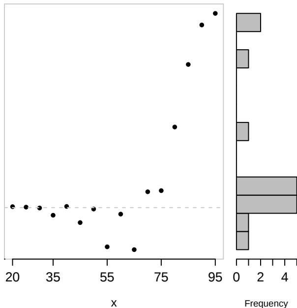
Residual plot
