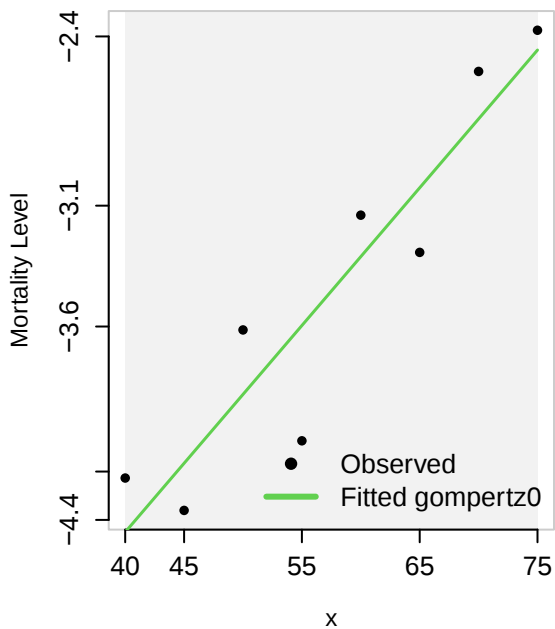
Observed vs. Fitted Gompertz law
