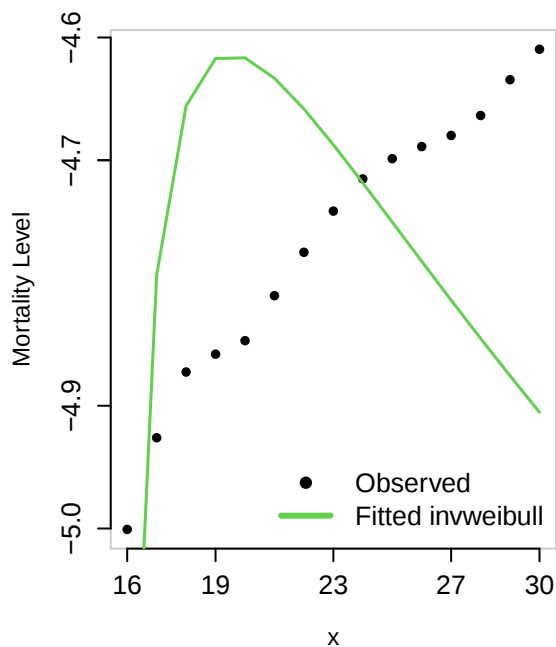
Observed vs. Fitted Inverse-Weibull law
