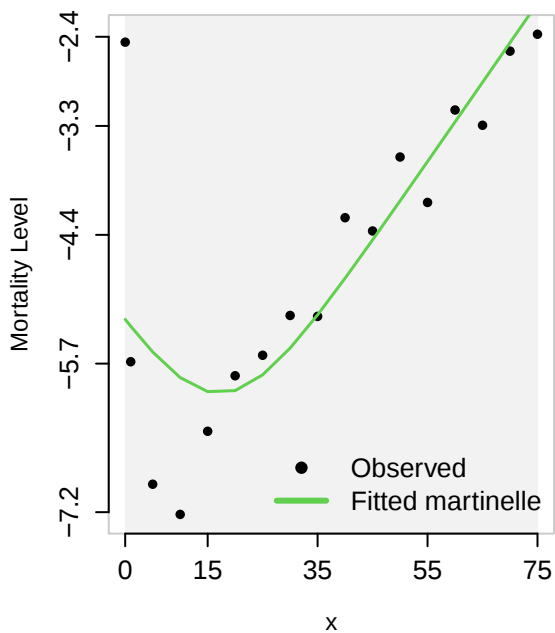
Observed vs. Fitted Martinelle law
