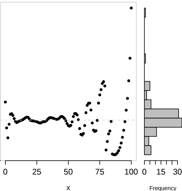
Residual plot
