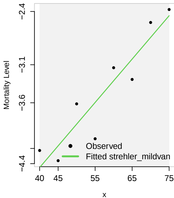
Observed vs. Fitted Strehler–Mildvan law
