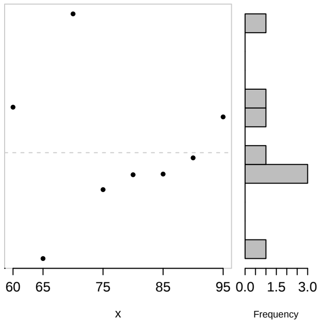
Residual plot
