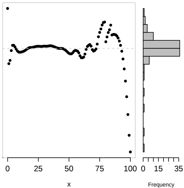
Residual plot
