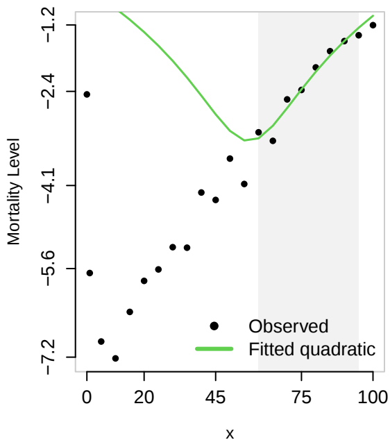
Observed vs. Fitted Quadratic law
