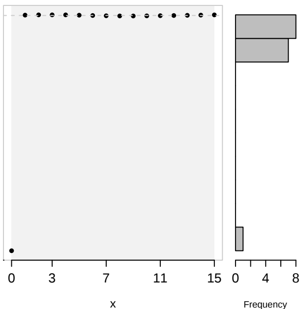
Residual plot
