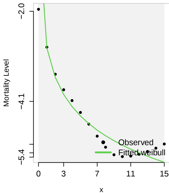
Observed vs. Fitted Weibull law
