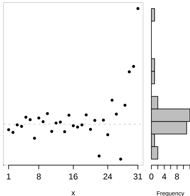
Residual plot
