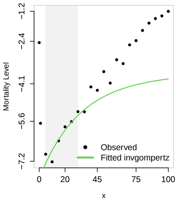
Observed vs. Fitted Inverse-Gompertz law
