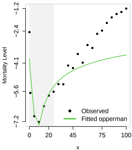
Observed vs. Fitted Opperman law
