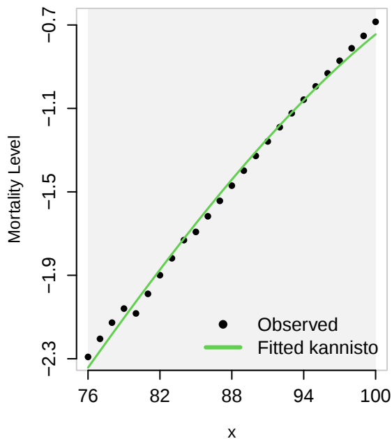
Observed vs. Fitted Kannisto law
