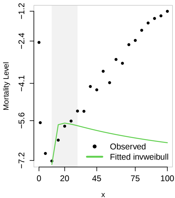
Observed vs. Fitted Inverse-Weibull law
