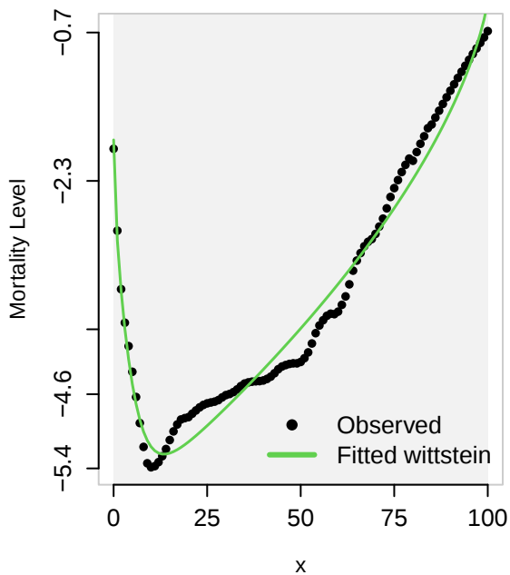
Observed vs. Fitted Wittstein law
