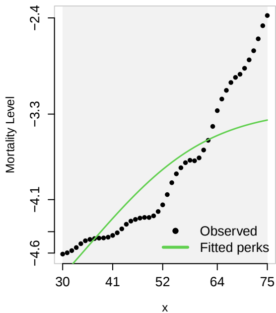
Observed vs. Fitted Perks law
