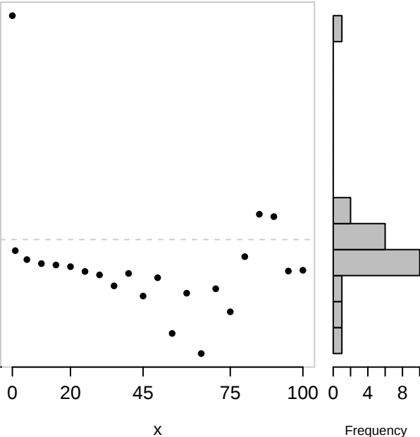
Residual plot
