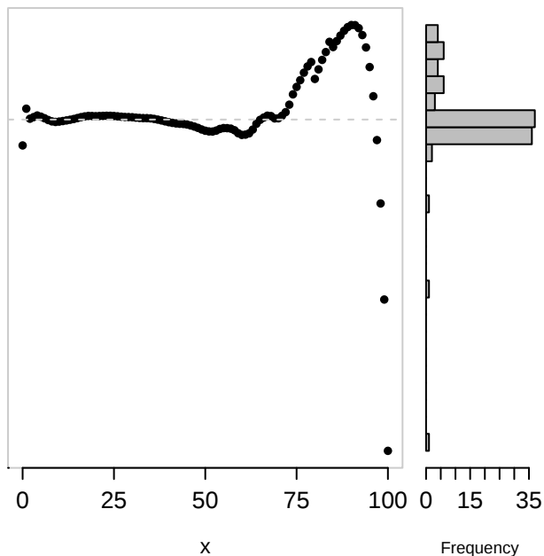
Residual plot
