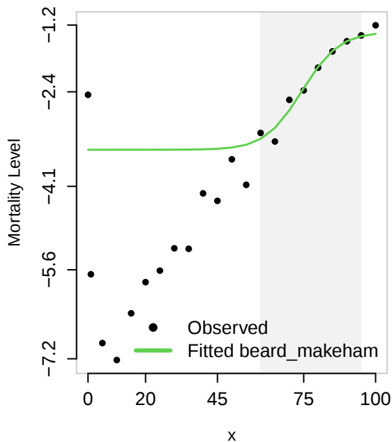
Observed vs. Fitted Beard–Makeham law
