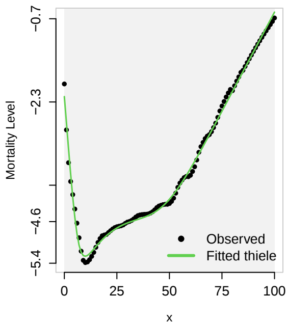
Observed vs. Fitted Thiele law
