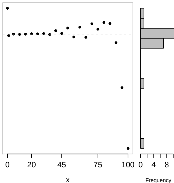
Residual plot
