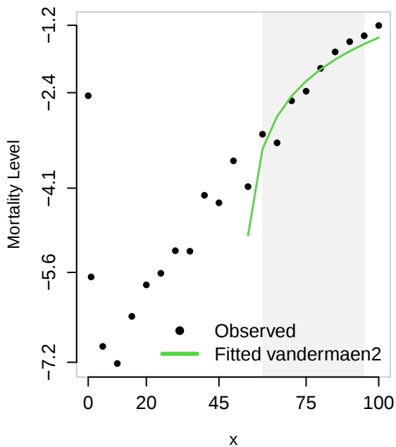
Observed vs. Fitted Van der Maen law
