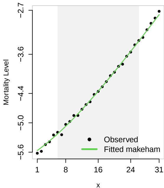
Observed vs. Fitted Makeham law
