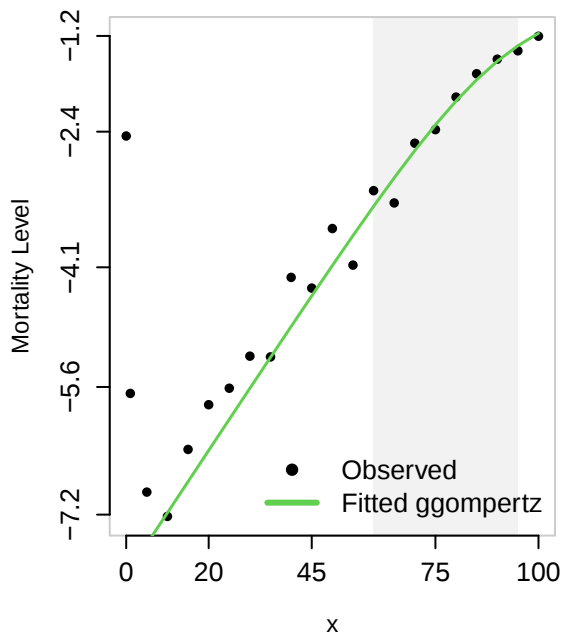
Observed vs. Fitted Gamma-Gompertz law
