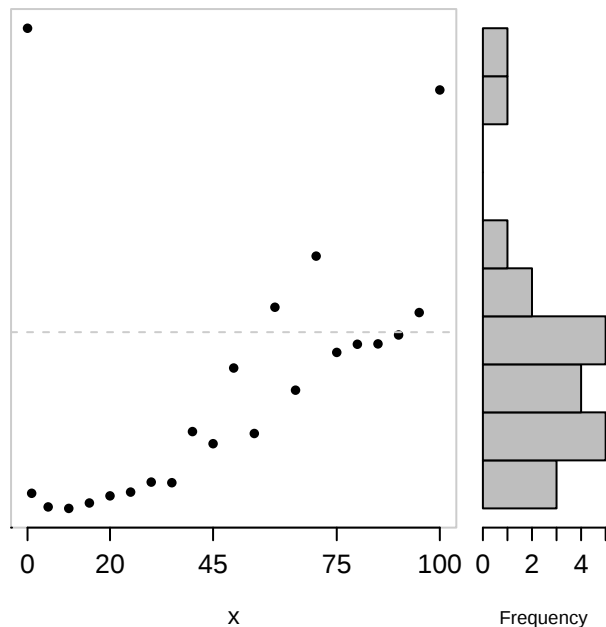
Residual plot
