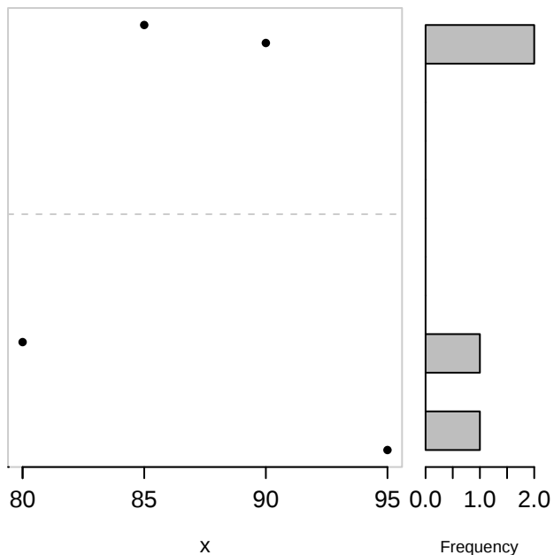
Residual plot
