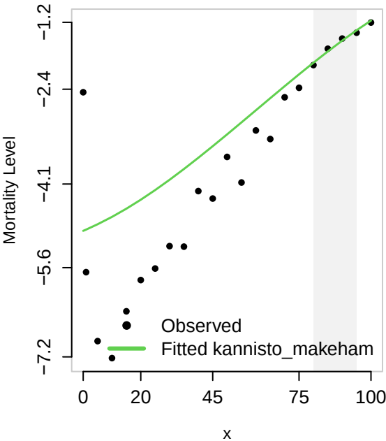
Observed vs. Fitted Kannisto–Makeham law
