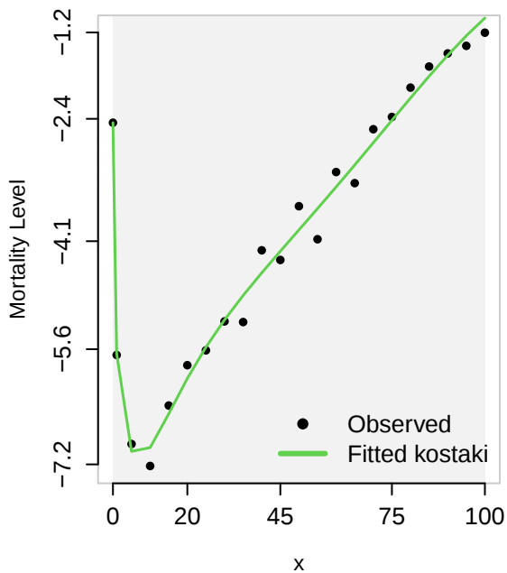
Observed vs. Fitted Kostaki law
