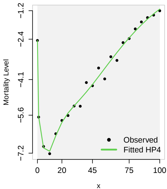
Observed vs. Fitted Heligman–Pollard law
