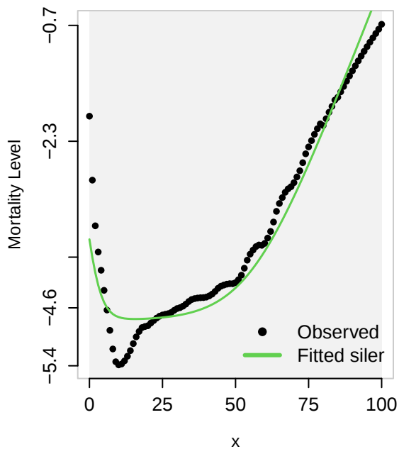
Observed vs. Fitted Siler law
