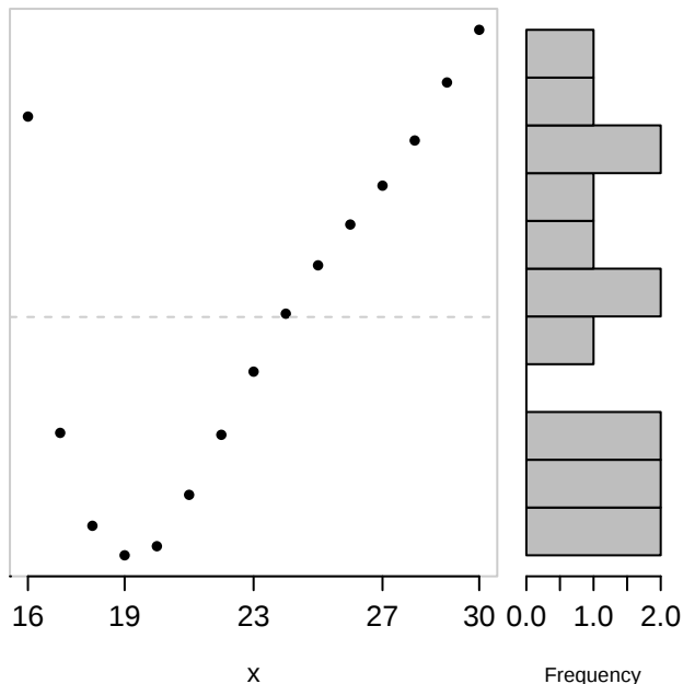
Residual plot
