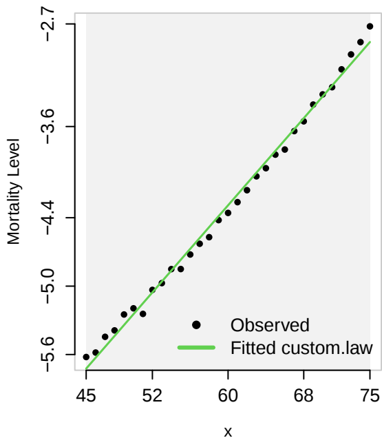
Observed vs. Fitted Custom Mortality law
