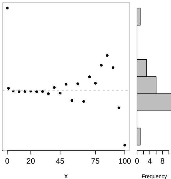
Residual plot
