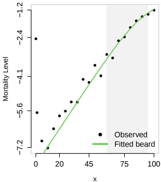
Observed vs. Fitted Beard law
