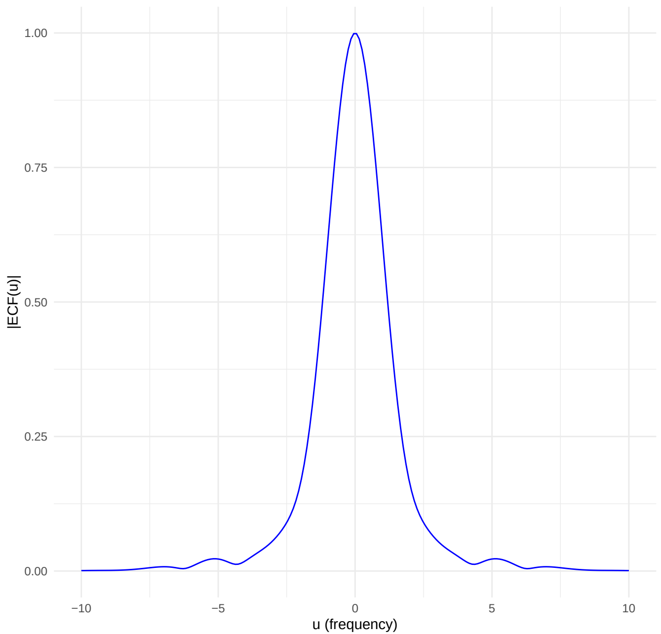
Empirical Characteristic Function (Kernel Smoothed)
