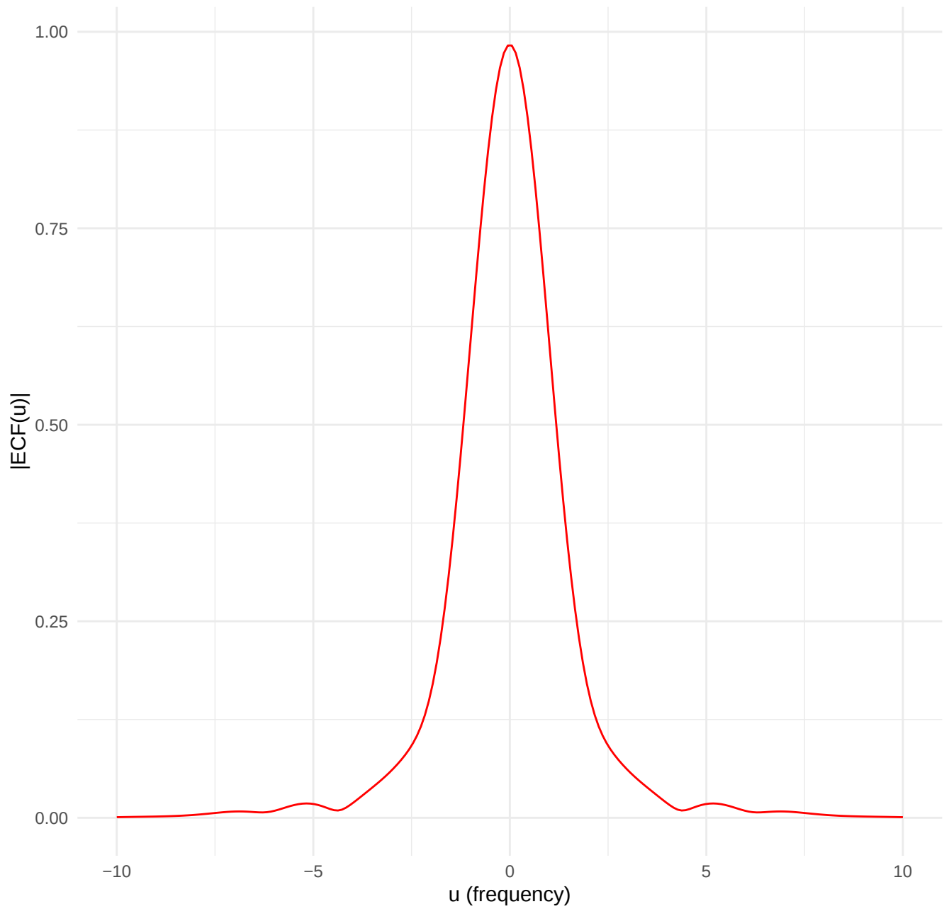
Empirical Characteristic Function (Recursive Smoothed)
