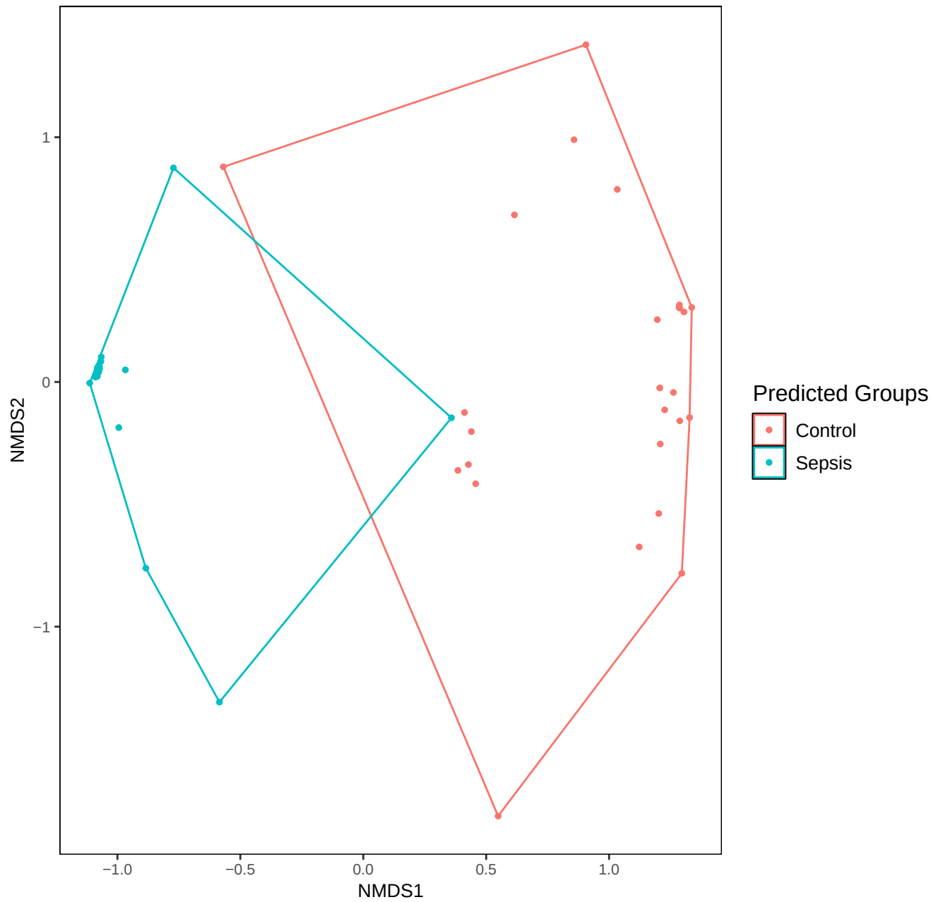
NMDS visualization
