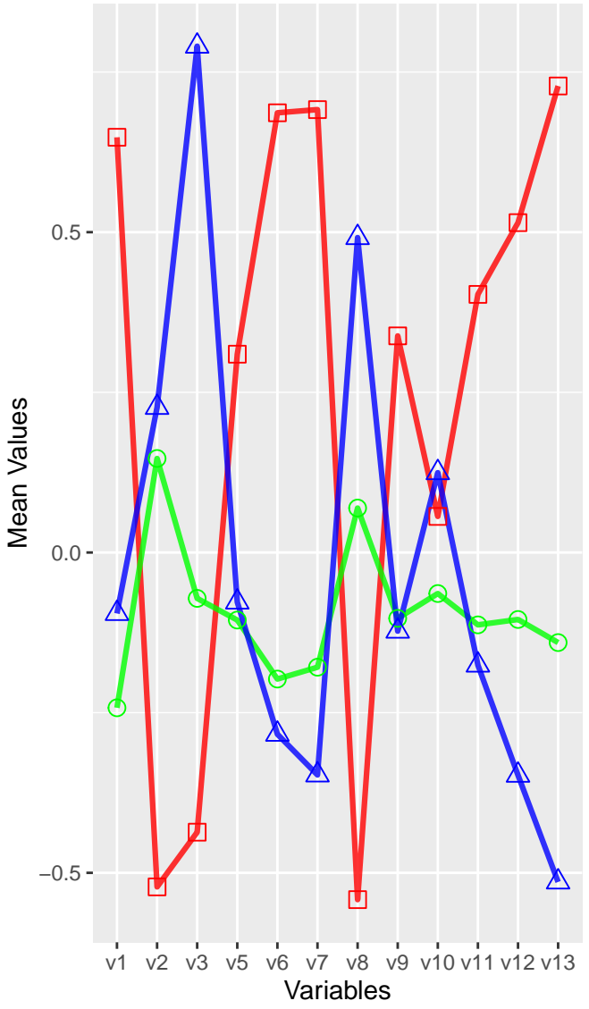
Mean Value Parallel Coordinates Plot
