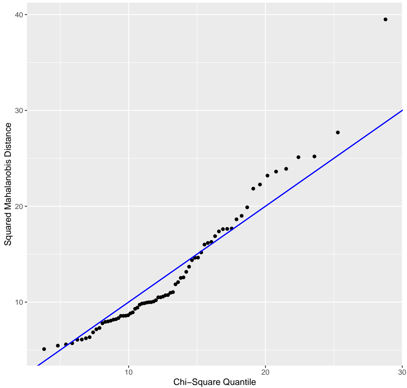
Chi-Square Q-Q plot
