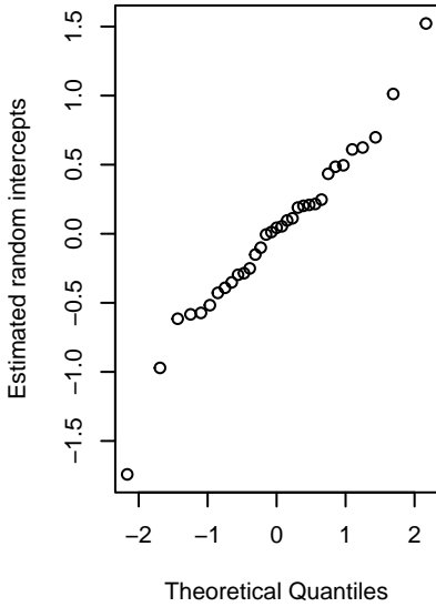
Random intercepts
