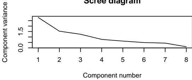
Scree diagram
