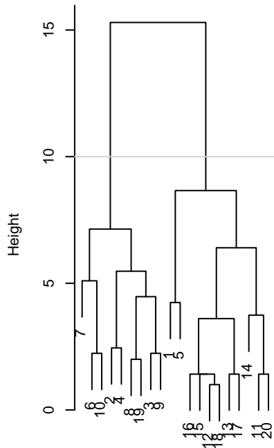
Complete
