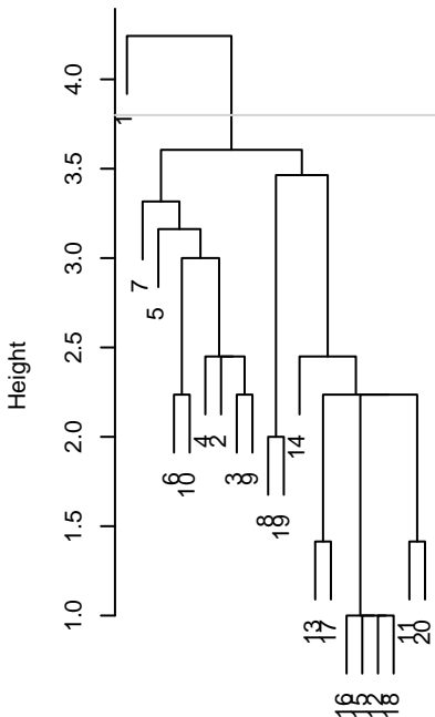
Single
