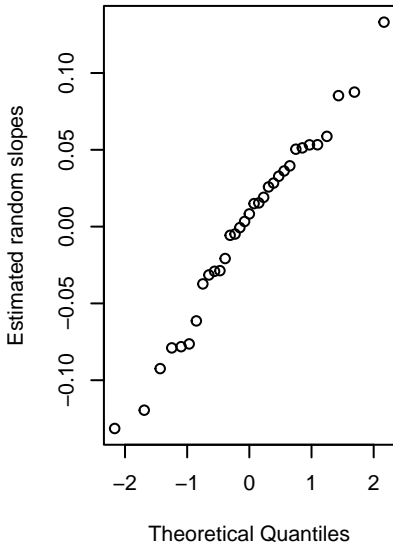
Random slopes
