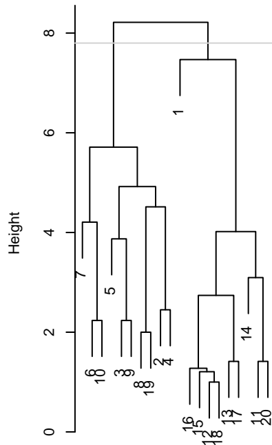
Average
