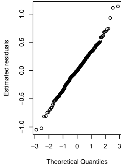
Residuals
