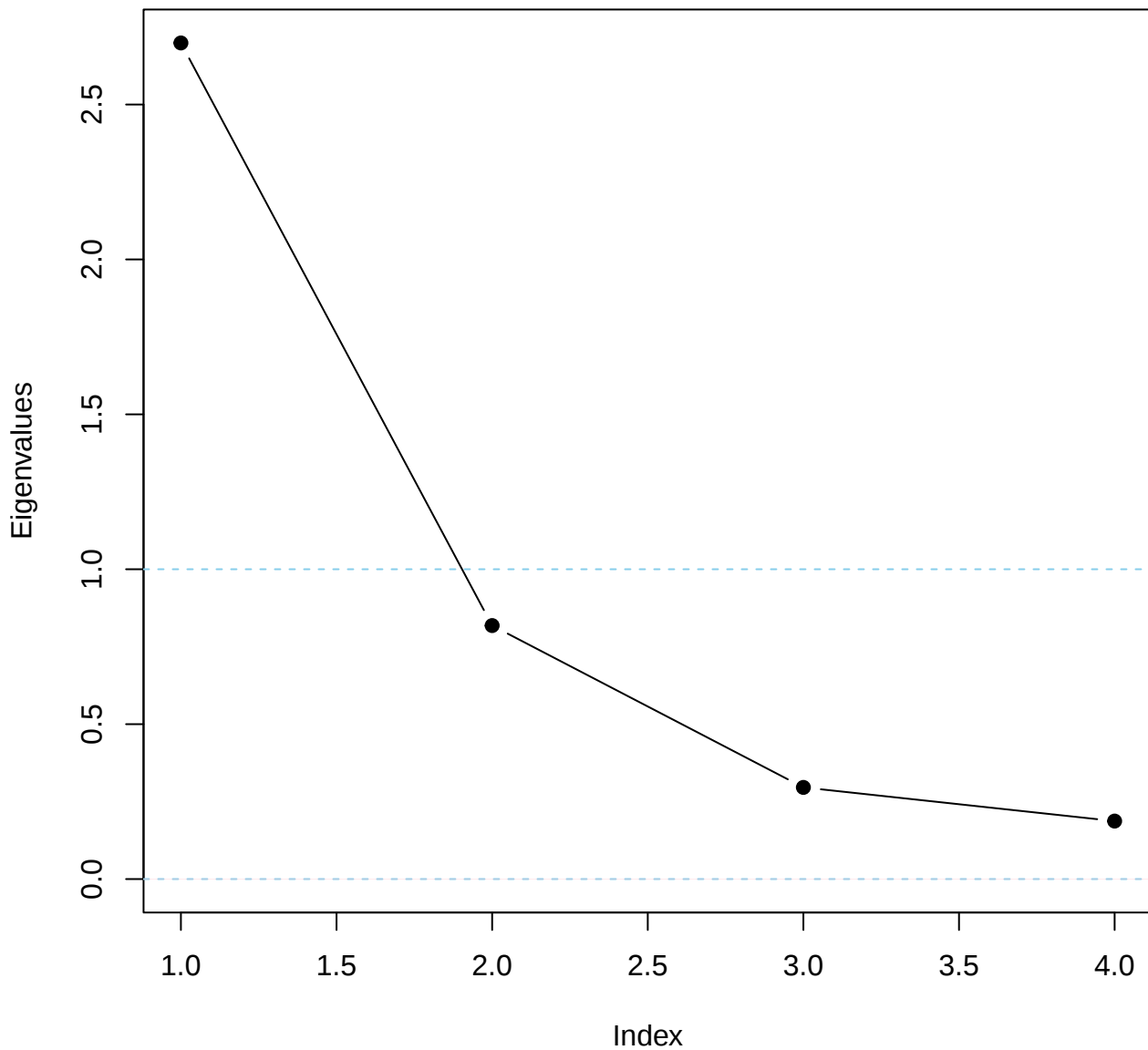
Scree Plot: correlationMatrix
