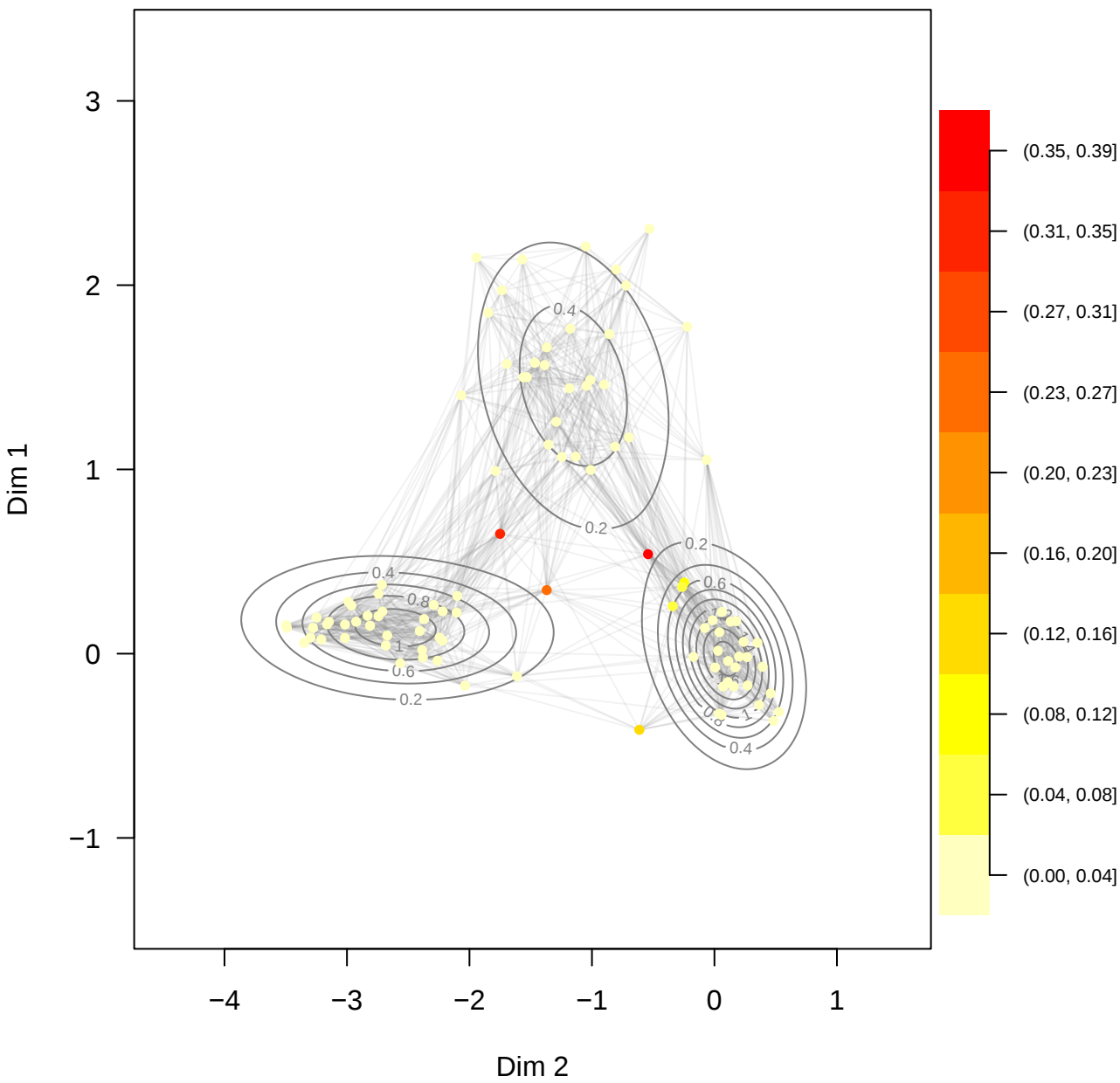
Latent Space Network Clustering – Actor-specific Clustering Uncertainty
