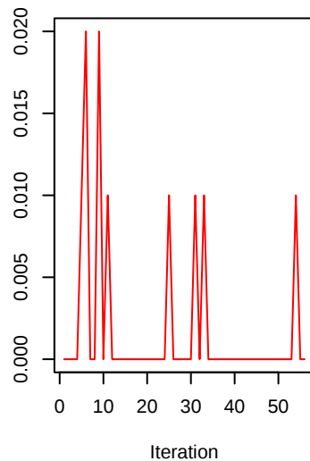
CER current vs. previous iteration
