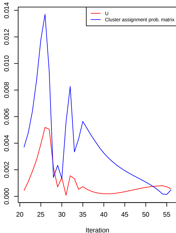
Abs diff. cumulative average
