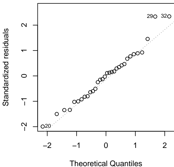
Q-Q Residuals
