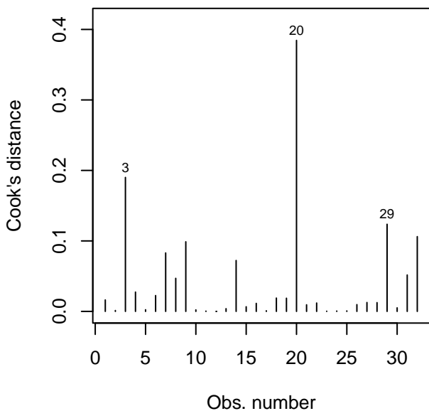
Cook's distance
