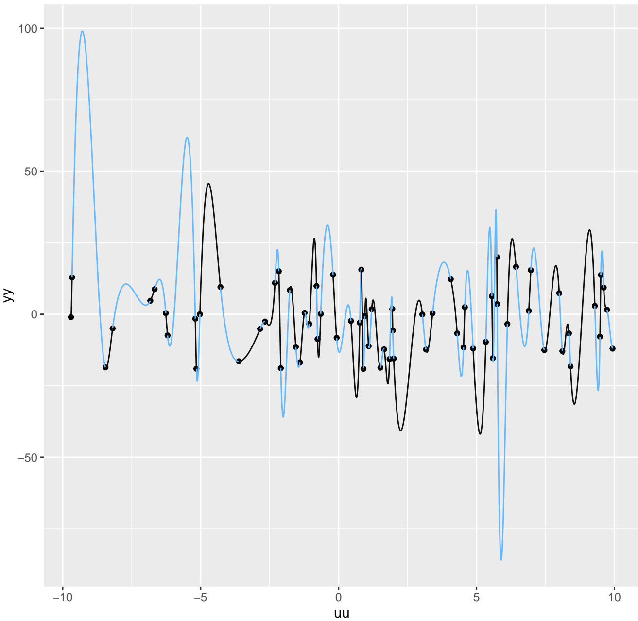
68-component non-uniform interpolation spline
