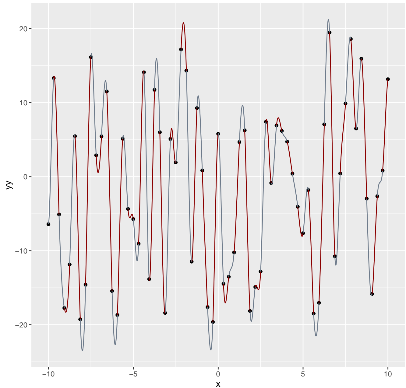
64-component uniform interpolation spline
