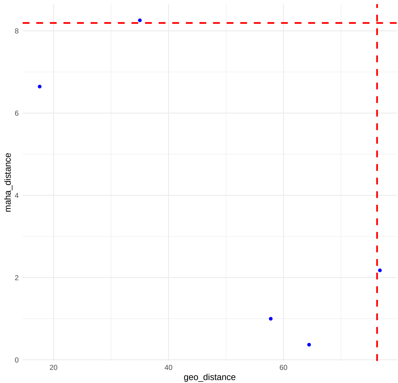
Scatter Plot 1
