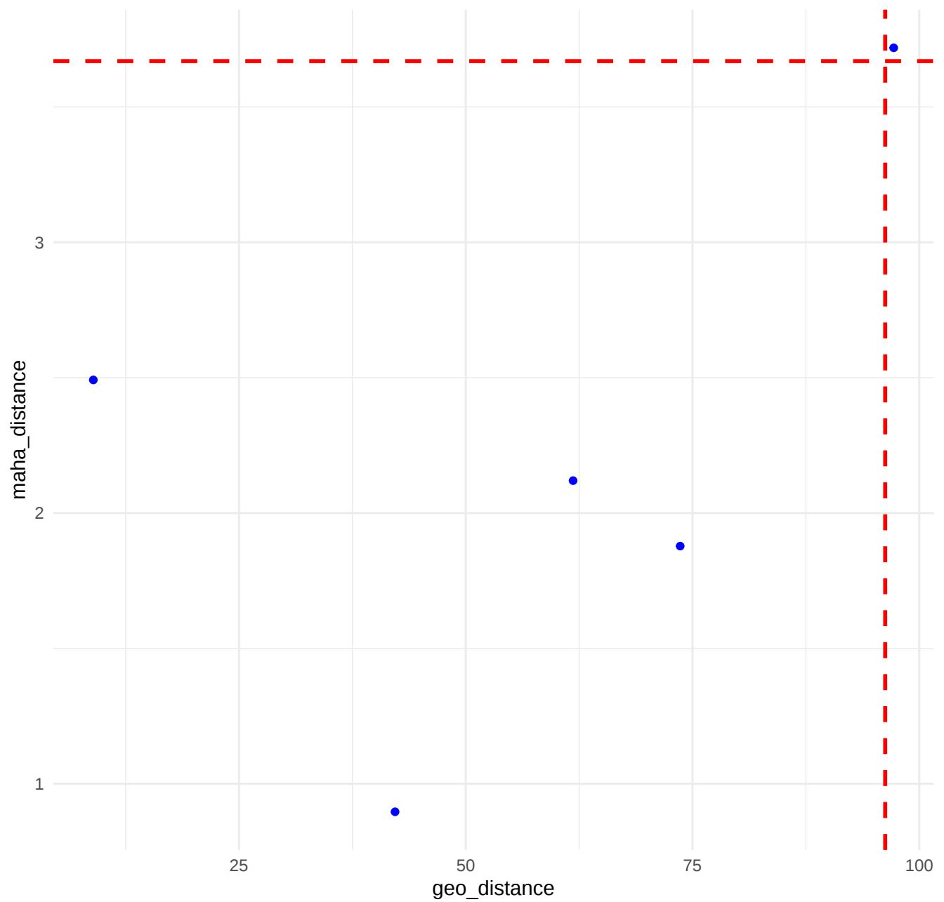
Scatter Plot 1
