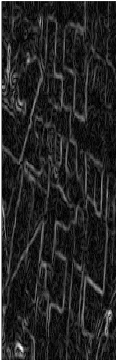
bandwidth=5
