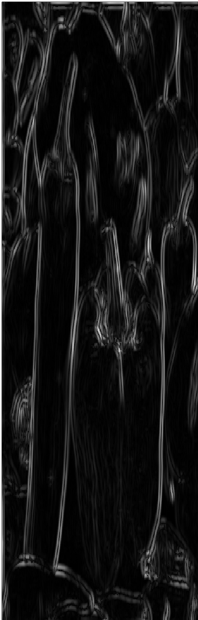
bandwidth=7
