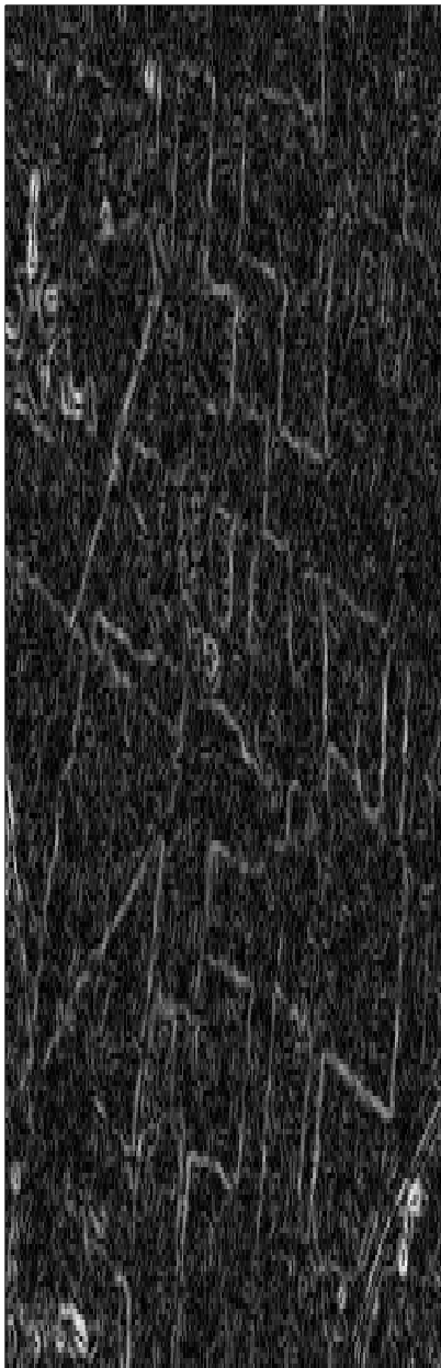
bandwidth=3
