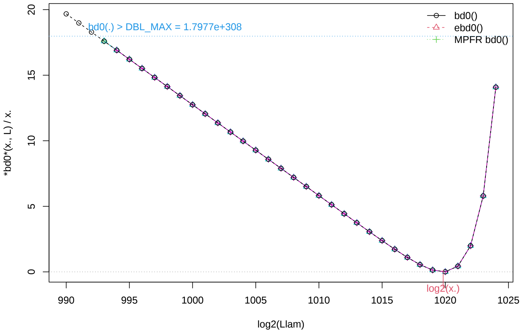
ebd0(x., Lam) and bd0(*) for x= 1e+307 *and* larg Lam
