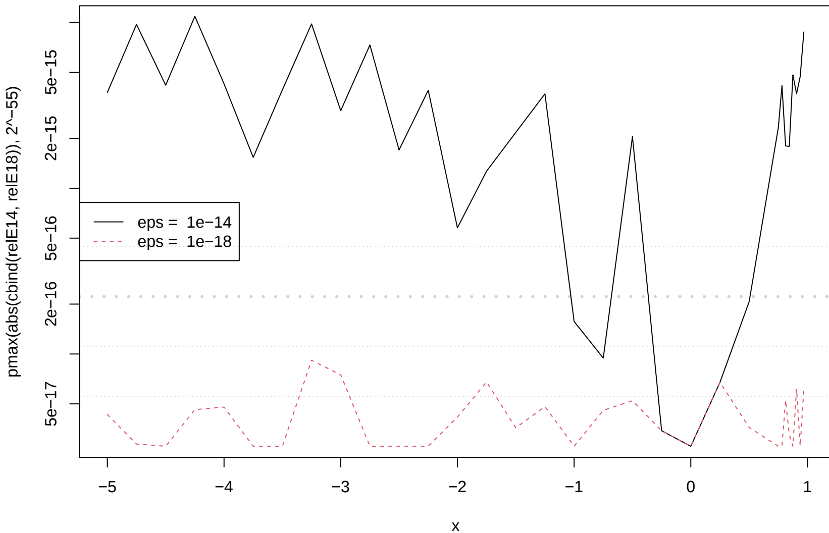
|relative Errors| (wrt mpfr precBits = 512) of \log_{cf}(x, 2, 3, \text{eps} = *)
