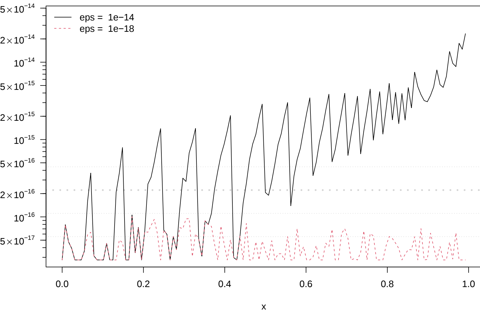
logcf(x, 2,3, eps = *): |relative Errors| wrt mpfr precBits = 512
