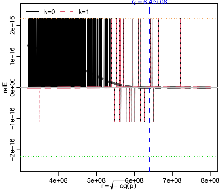
Relative error of qnormAsymp(*, k) around r_0 = 6.4e+08 for k = 0:1
