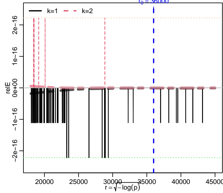
Relative error of qnormAsymp(*, k) around r_0 = 36000 for k = 1:2
