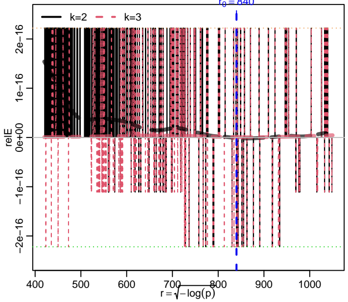
Relative error of qnormAsymp(*, k) around r_0 = 840 for k = 2:3
