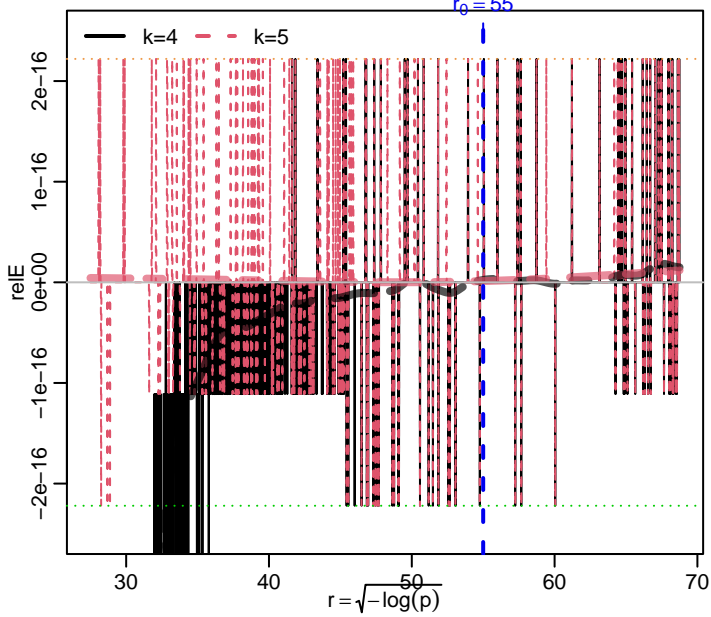
Relative error of qnormAsymp(*, k) around r_0 = 55 for k = 4:5
