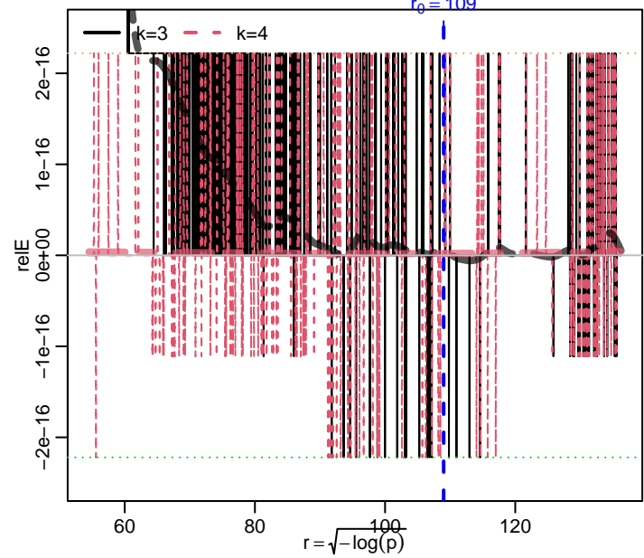
Relative error of qnormAsymp(*, k) around r_0 = 109 for k = 3:4
