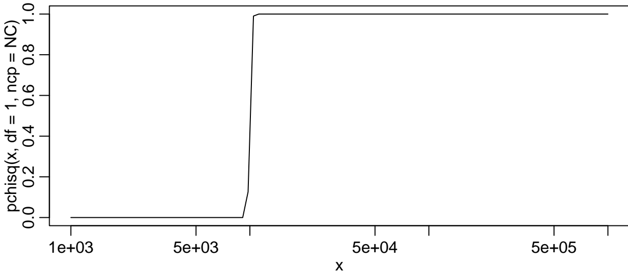
CDF ncp = 10000
