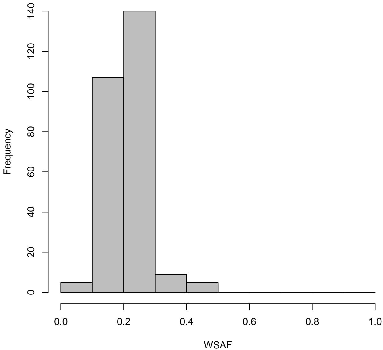
Histogram 0 < \text{WSAF} < 1
