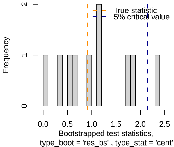
Bootstrap Regression Test
