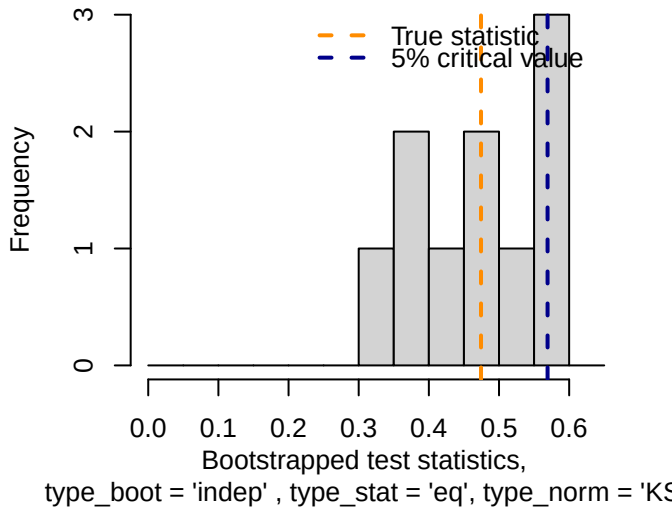
Bootstrap Independence Test
