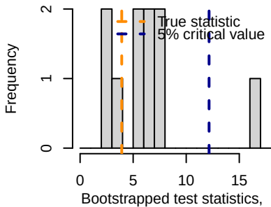
Bootstrap Independence Test
