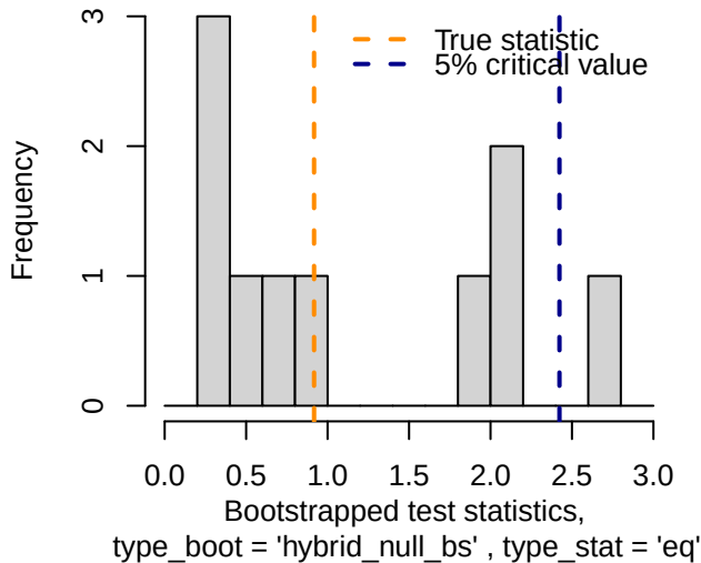
Bootstrap Regression Test
