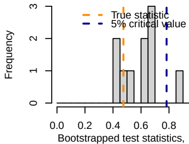
Bootstrap Independence Test
