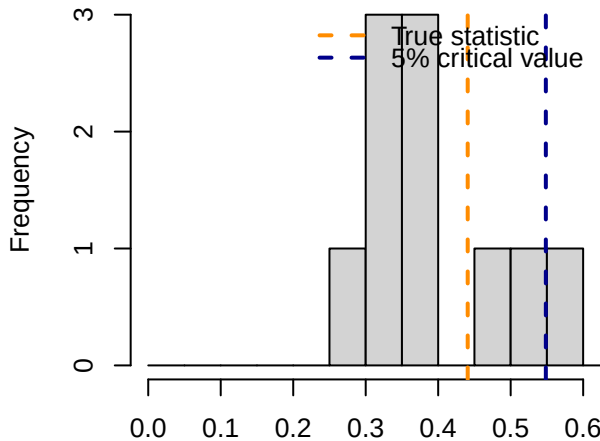
Bootstrap GoF Test
