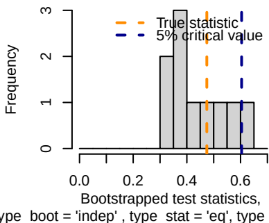
Bootstrap Independence Test
