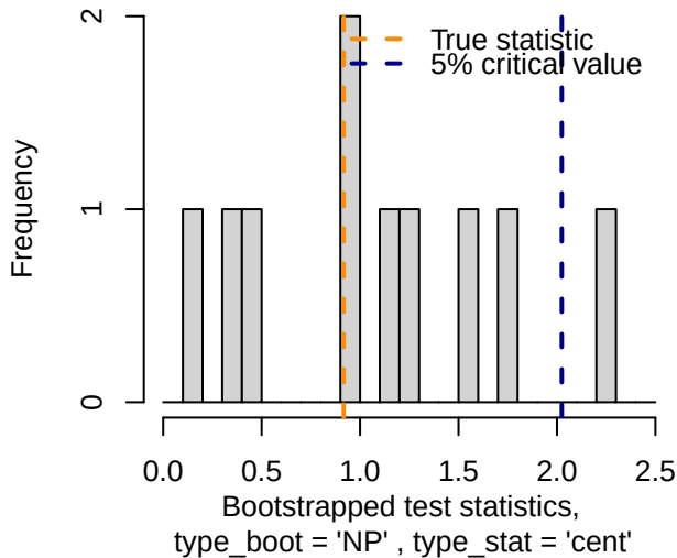
Bootstrap Regression Test
