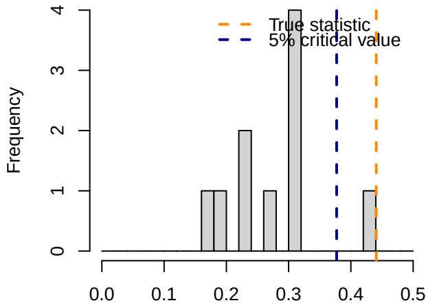
Bootstrap GoF Test
