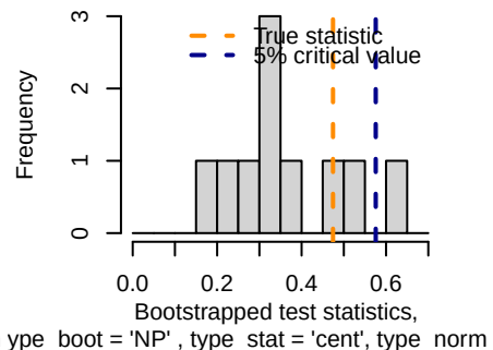
Bootstrap Independence Test
