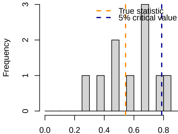
Bootstrap GoF Test
