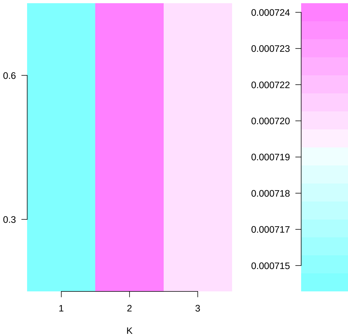
CV MSPE Plot
